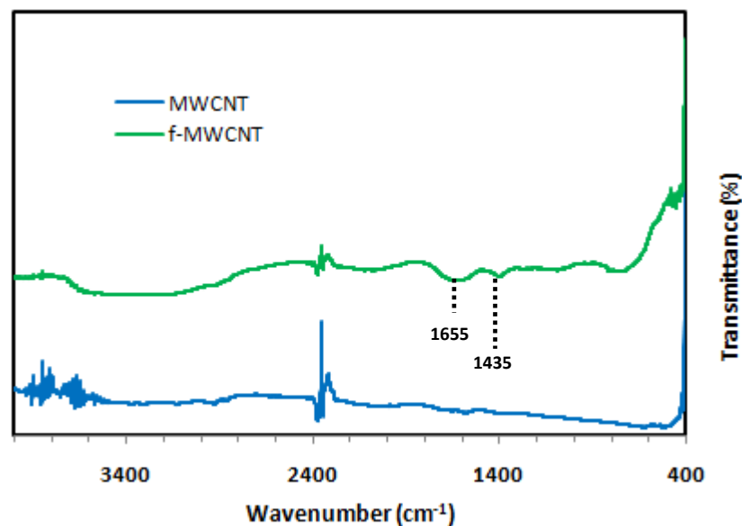
Fig S1. FTIR spectra for MWCNT and f-MWCNT.
