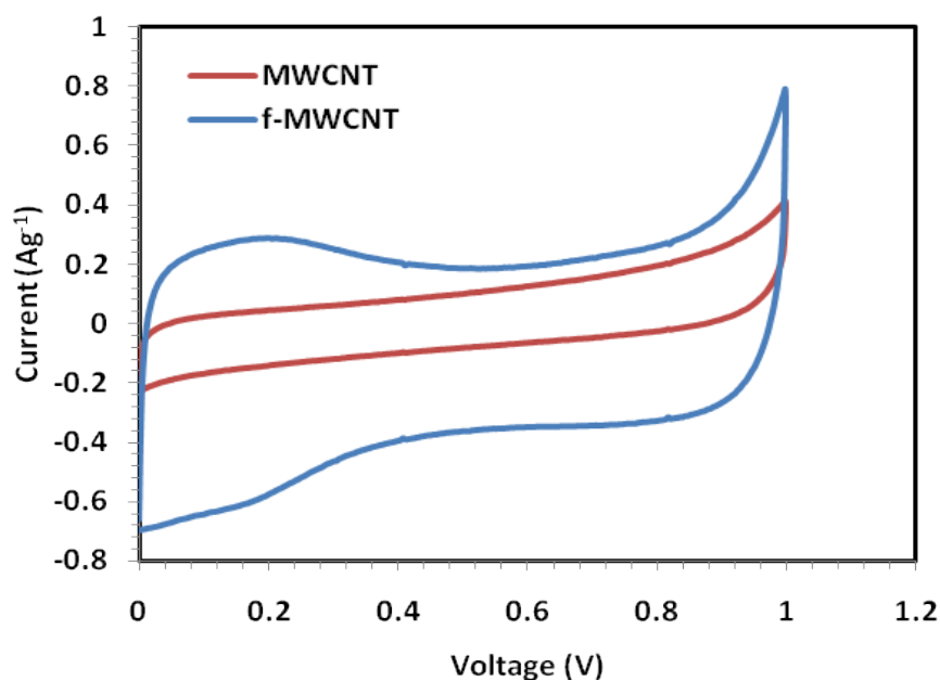
Fig S2. CV curves of MWCNT and f-MWCNT at scan rate of 5 mVs -1 .
