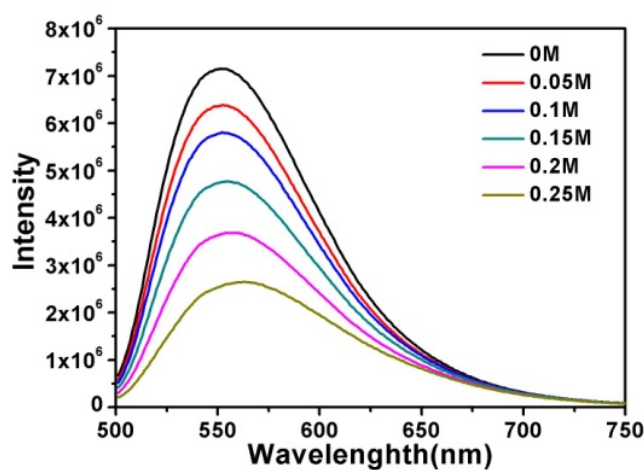
Figure S1. The fluorescence spectra of CDs about quenching addition of different concentrations of 2, 4-dinitrotoluene.
