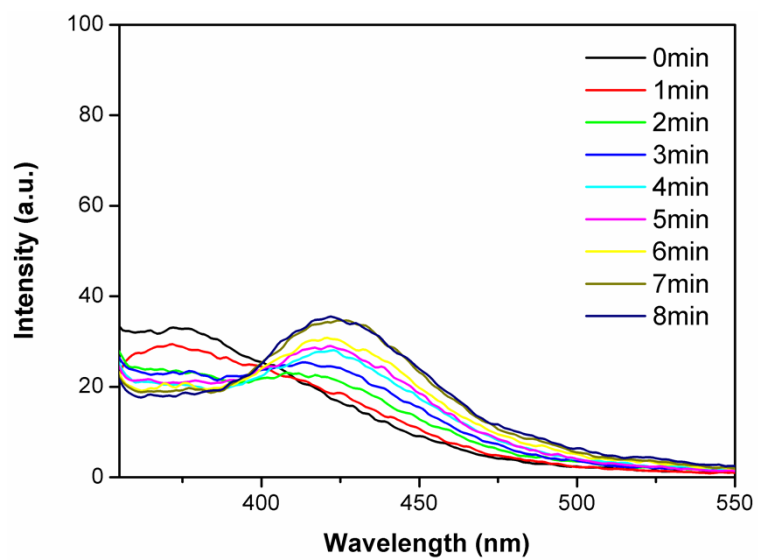
Figure S3 •OH-trapping PL spectrum of Pt/Ag 3 PO 4 heterostructures under visible light irradiation ( \lambda > 420 nm).
