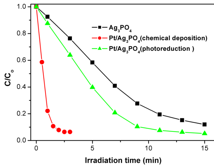
Figure S2 Effect of metal deposition method on the photocatalytic activity toward MO degradation.
