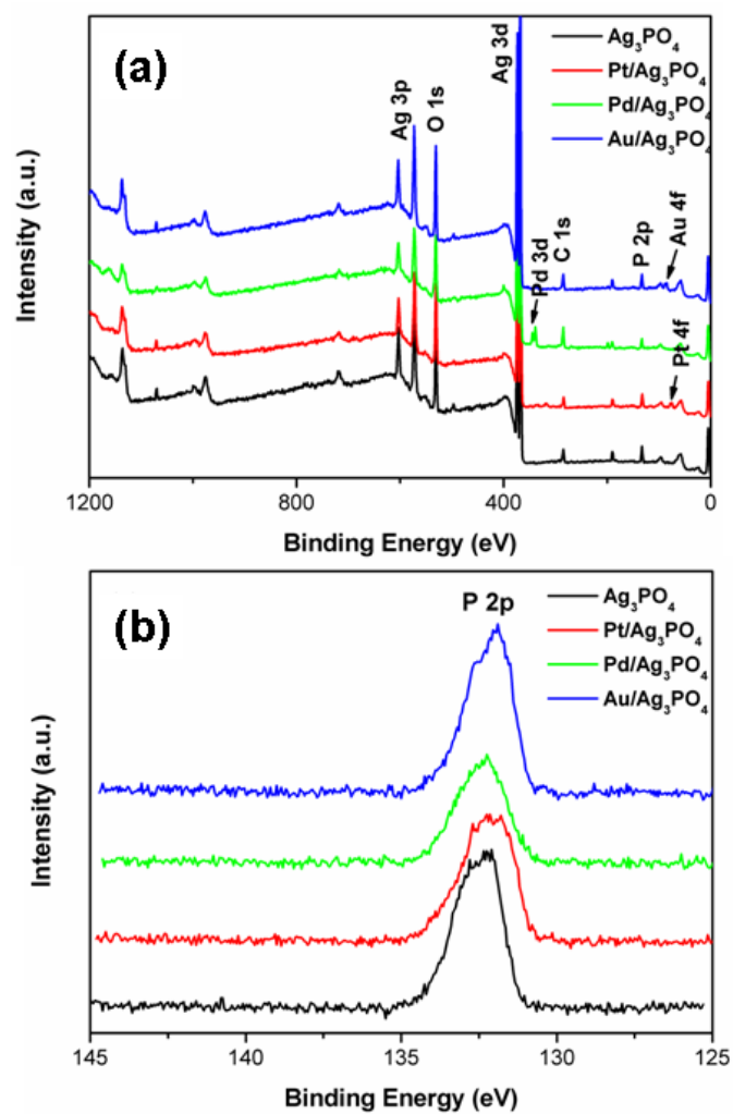
Figure S1 XPS spectra of M/ \text{Ag}_3\text{PO}_4 and \text{Ag}_3\text{PO}_4 . (a) full spectra, (b) P 2p spectra.
