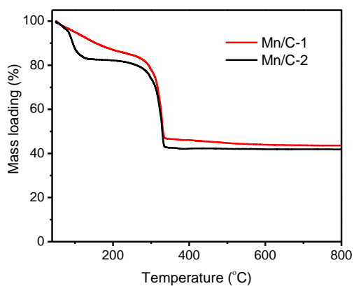
Figure S2. The TGA curves of Mn/C-1 and Mn/C-2.
