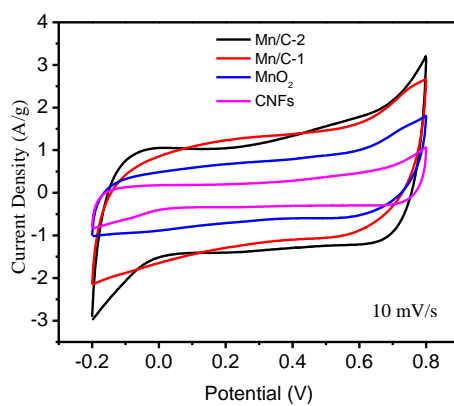
Figure. S3. CV curves at 10 mV/s for pure CNFs, \text{MnO}_x , Mn/C-1 and Mn/C-2
