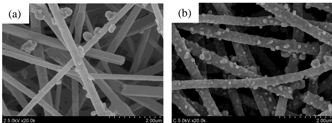
Figure. S4 SEM images of (a) Mn/C-1 and (b) Mn/C-2 tested at 1 A/g after 2000 cycles
