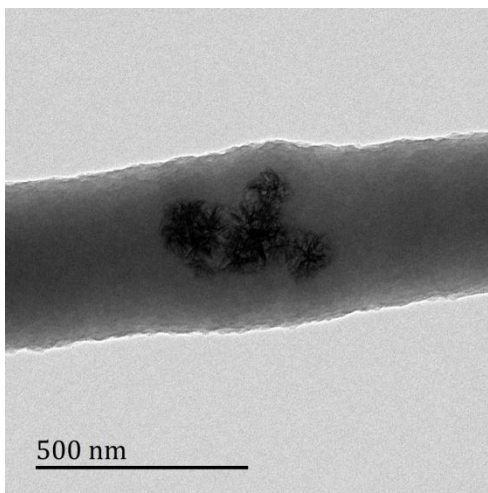
Figure S1. TEM image of \text{MnO}_2 in Mn/C-1 nanofibers with a high magnification.
