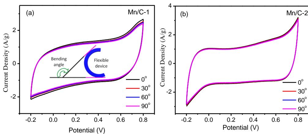
Figure S6. CV curves of (a) Mn/C-1 and (b) Mn/C-2 tested at various bending angles.
