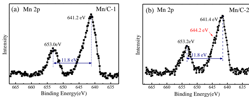
Figure. S5. XPS Mn 2p spectrum of Mn/C-1 and Mn/C-2 tested at 1 A/g after 2000 cycles
