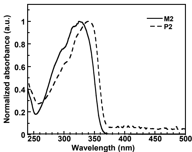
Fig. S2 Absorption spectra of M2 and P2 in dilute CH 2 Cl 2 solution.
