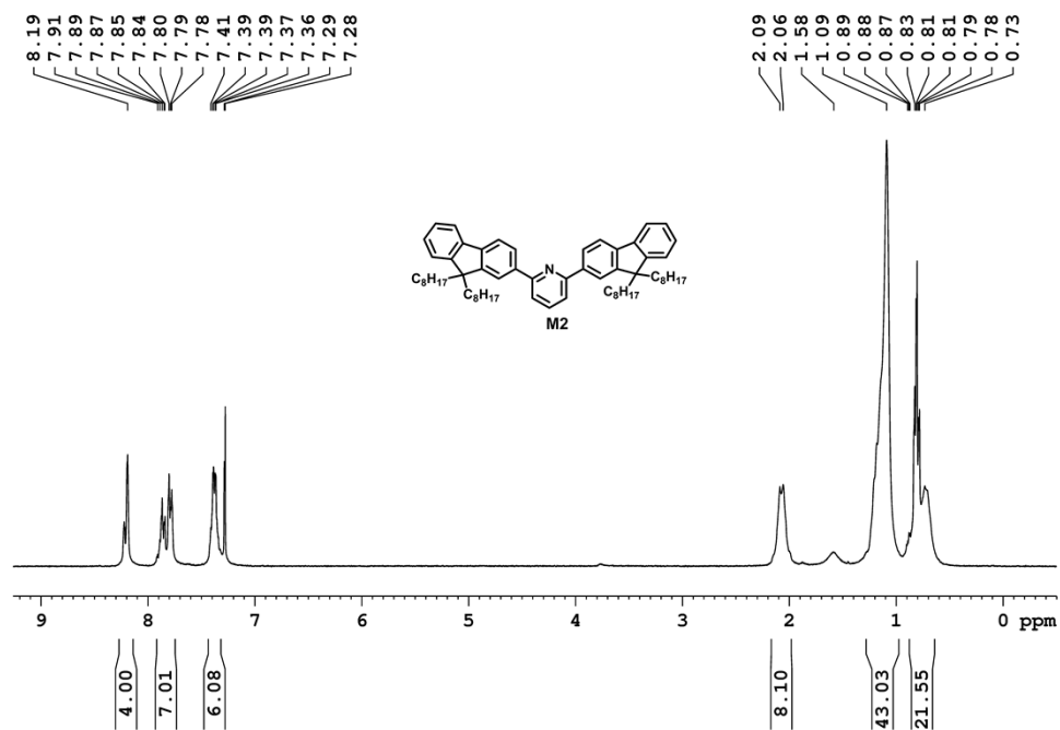
Fig. S5 ^1\text{H} NMR of M2 in \text{CDCl}_3 .
