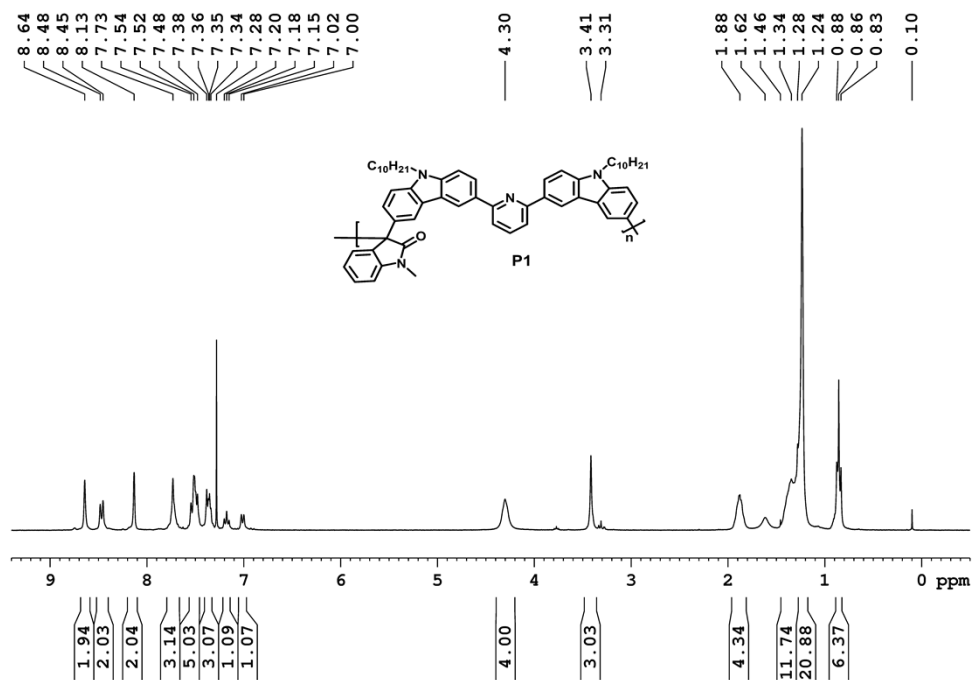
Fig. S4 ^1\text{H} NMR of P1 in \text{CDCl}_3 .
