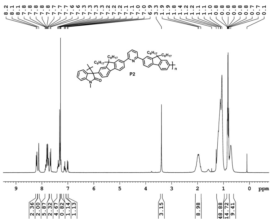
Fig. S6 ^1\text{H} NMR of P2 in \text{CDCl}_3 .
