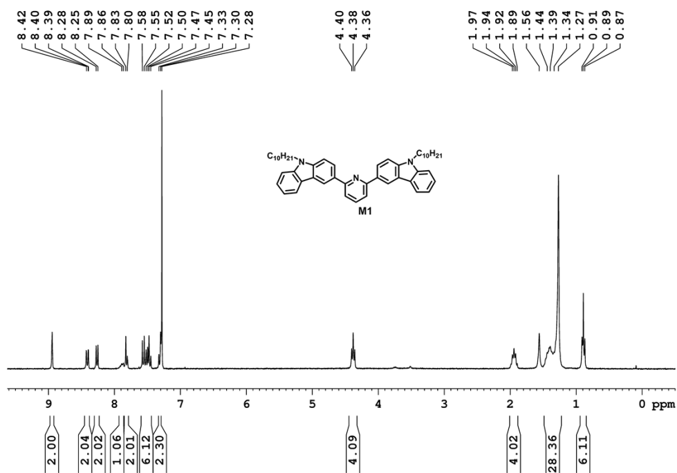
Fig. S3 ^1\text{H} NMR of M1 in \text{CDCl}_3 .
