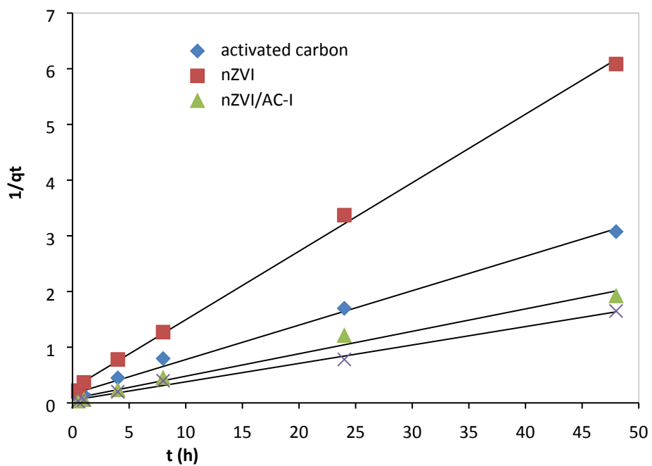
SI Fig.1: Linear plot second-order reaction model fitting
