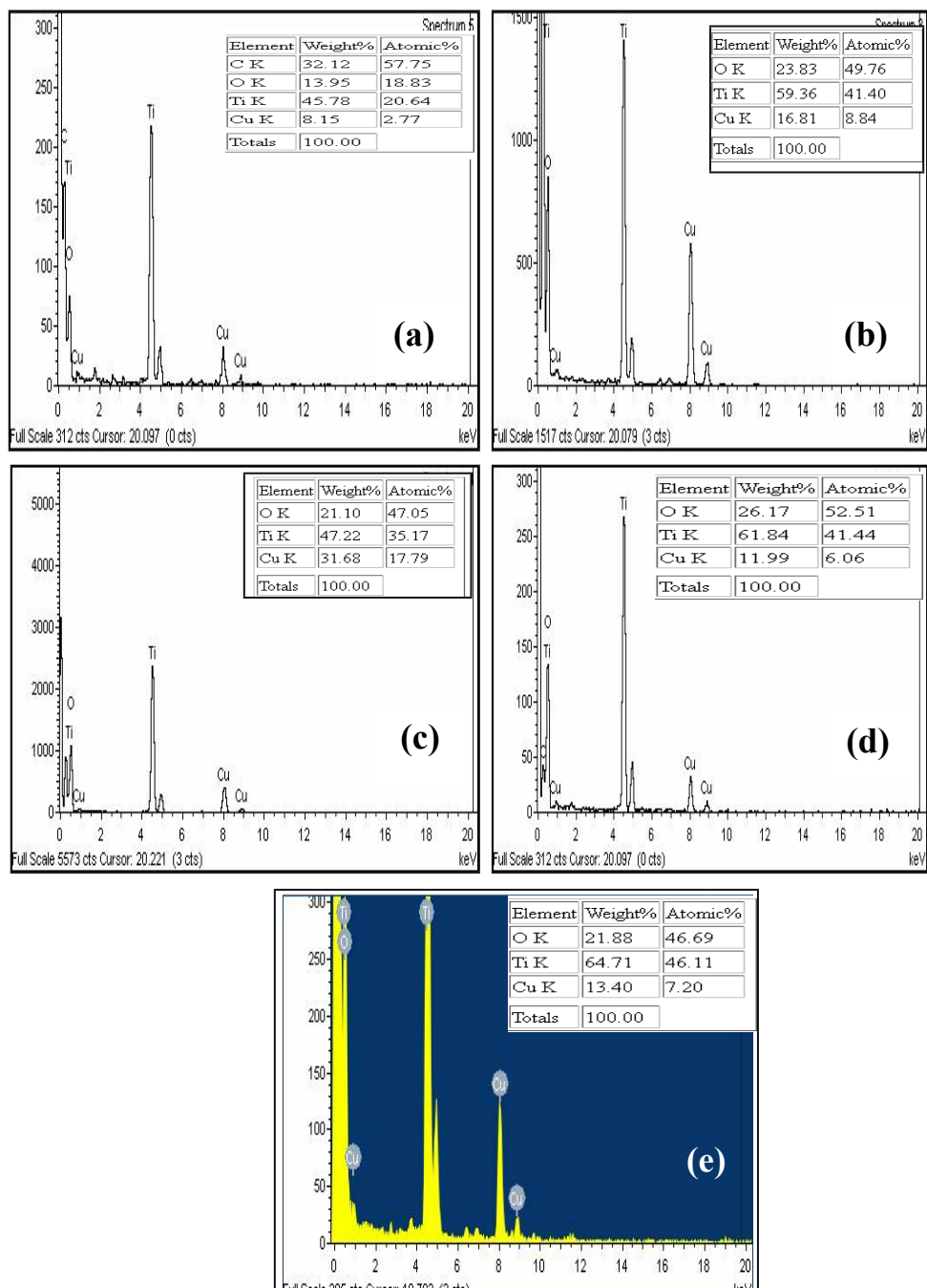
Fig. S2 EDS spectra of (a) native titania, (b) titania at 600°C and (e) chemical titania at 600°C.
