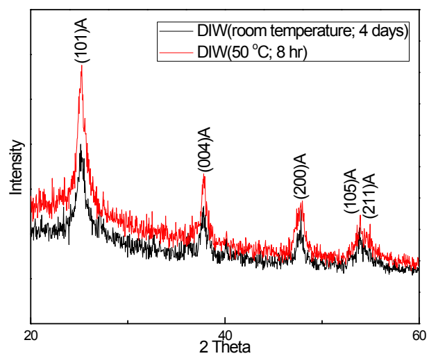
Fig. (S3) XRD pattern of water processed TNT at room temperature for 4 days and 50 °C for 8 h
