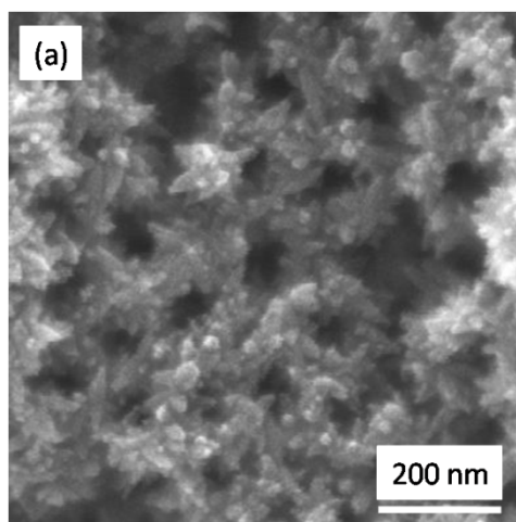
Fig. (S1) FESEM image of water processed TNT at room temperature for 4 days
