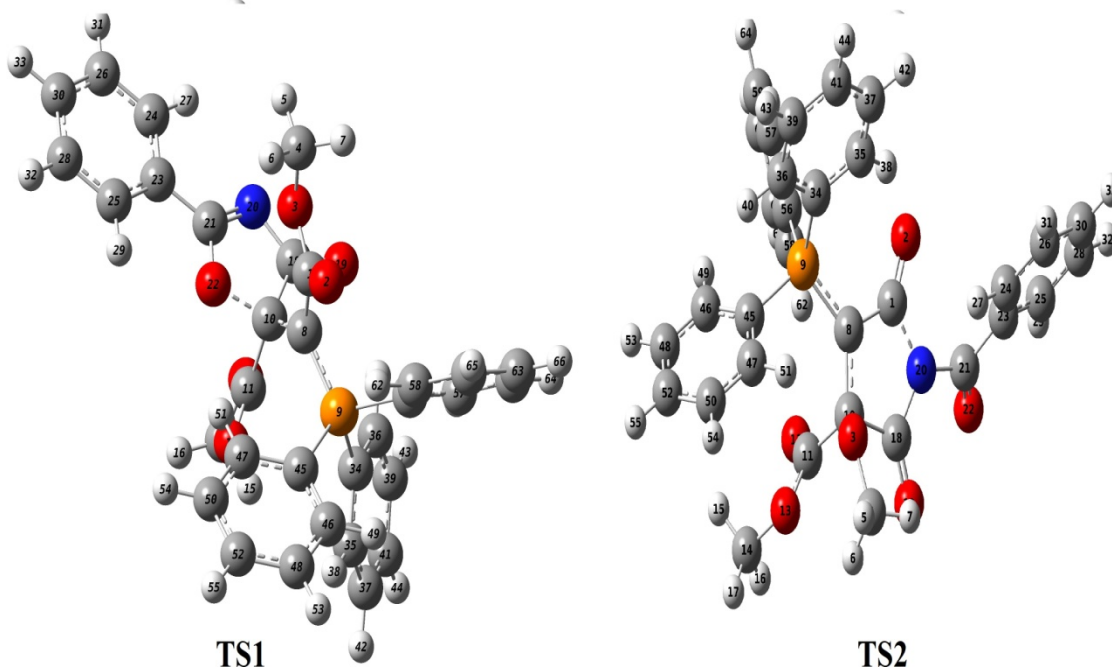
Figure S3. Optimized TS structures for routes 2 and 4, respectively, in the gas phase by the B3LYP/6-31G(d) functional.
