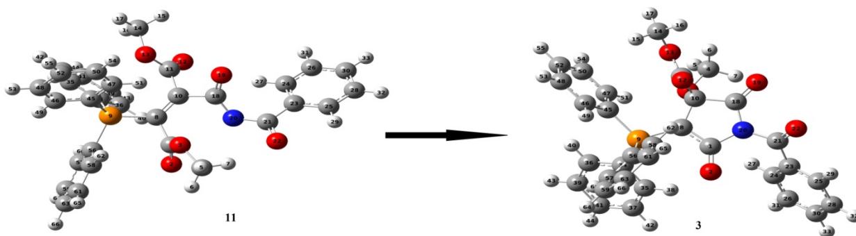
Figure S1. Optimized structures for mechanism 2 in the gas phase by the B3LYP/6-31G(d) functional
