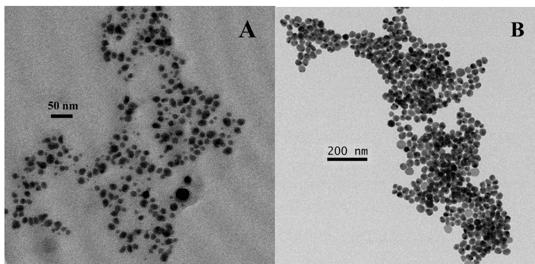
Figure S1 TEM images of DNA-Au hybrids, (A): Au: 15nm, (B): Au: 25nm
