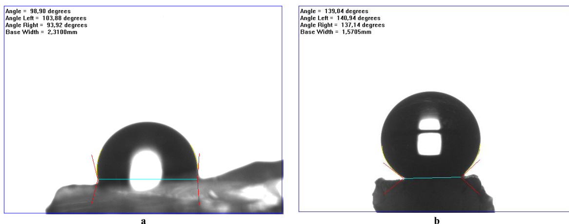
Fig. S1 The water sessile drop contact angles of AG-3 aerogels supercritically dried in CO 2 (a) and HFIP (b).
