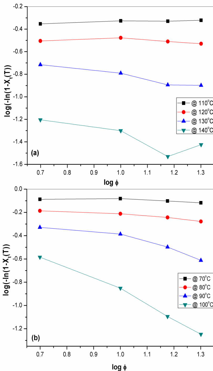
Fig S1: Ozawa plots for non-isothermal crystallization process for (a) pristine PVdF-HFP and (b) PVdF-HFP+ 10 wt.% BMIMBF 4
