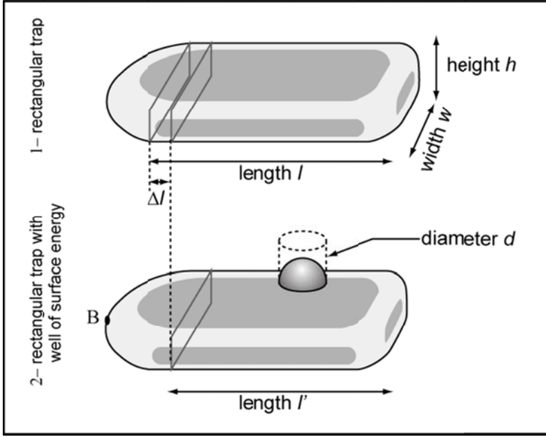
Figure. Definition of the parameters for estimating the added trapping energy allowed by using a well of surface energy.
