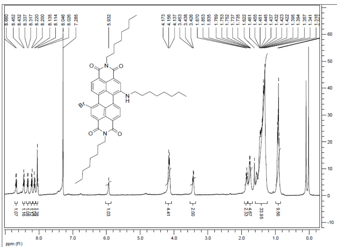
Figure d The 1 H-NMR chart of compound C3
