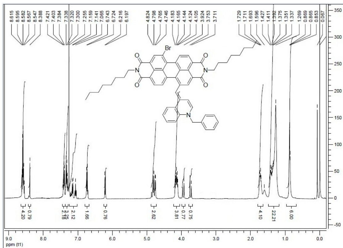
Figure c The 1 H-NMR chart of compound C2
