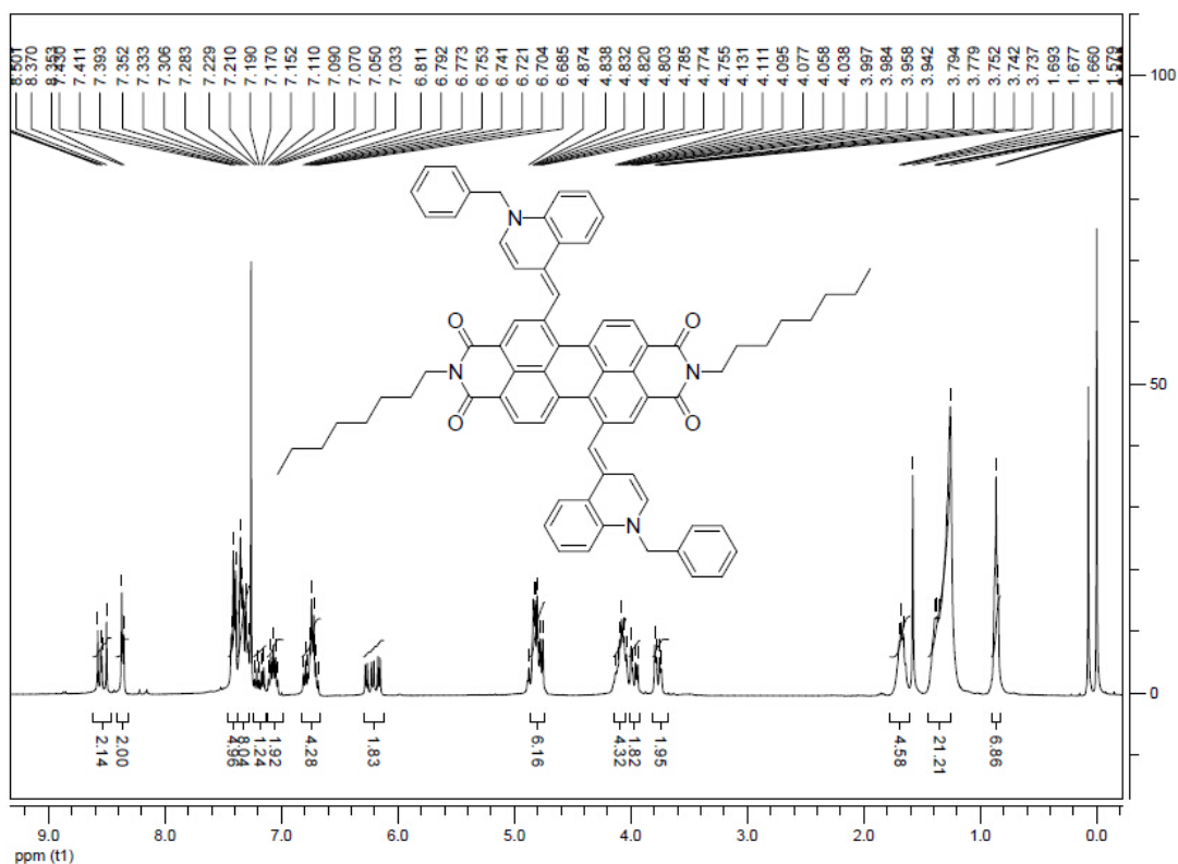
Figure b The 1 H-NMR chart of compound C1
