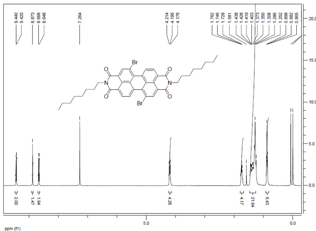
Figure a The 1 H-NMR chart of intermediate Br-PDI
