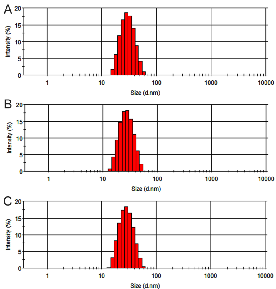
Figure S1 Particle size distribution of micelles (A), Dox-M (B) and Cur-M (C).
