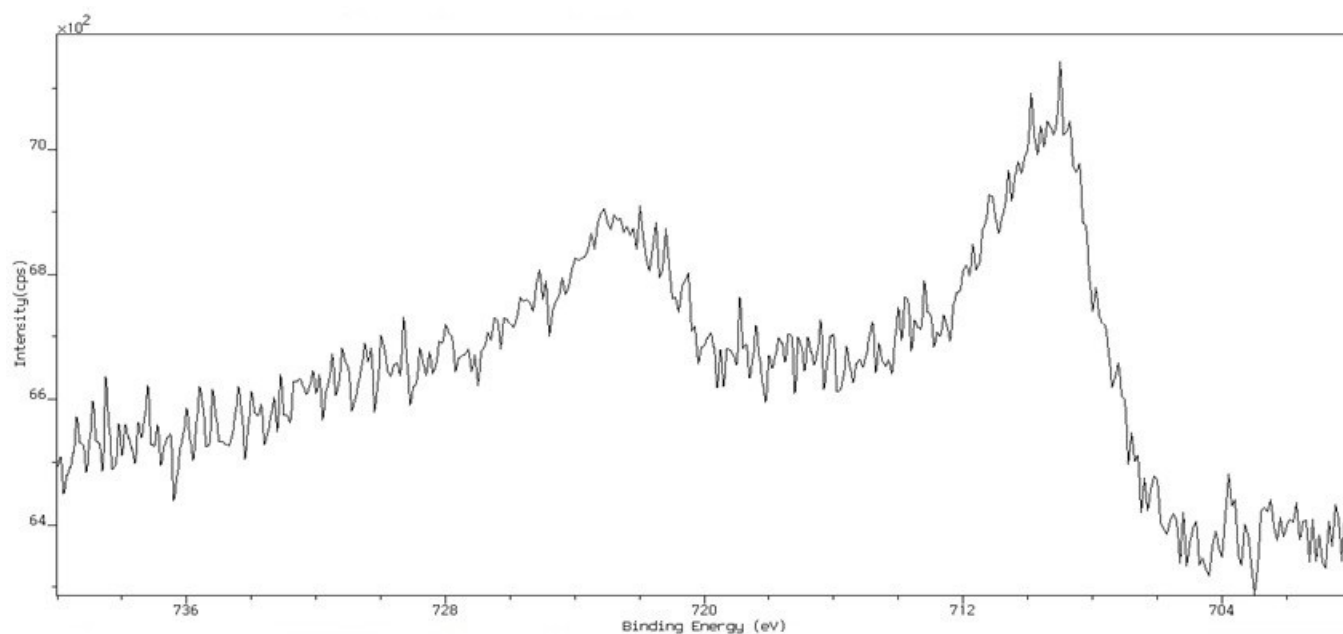
Figure 1. XPS of Fe-TiO 2 - Fe 2p
