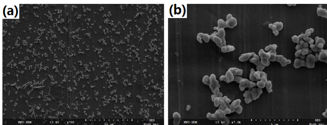
Fig S1: The SEM images of the Ag particles synthesized using the mixture of mPEG-5000 and PVP-29,000 homopolymer. (a) and (b) are the low and high-magnification SEM of the prepared PVP-Ag, respectively.
