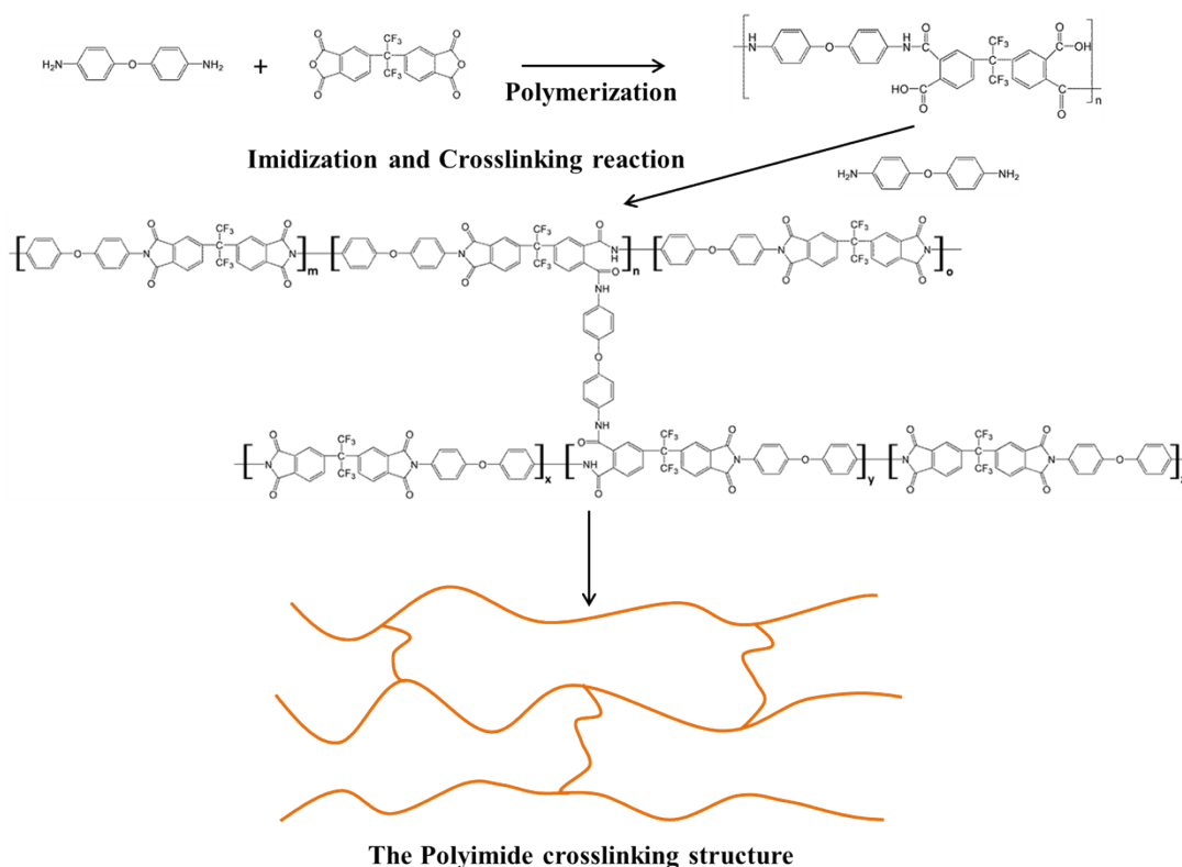
Fig. S1 The polymerization, imidization and crosslinking reaction mechanism of SPI.
