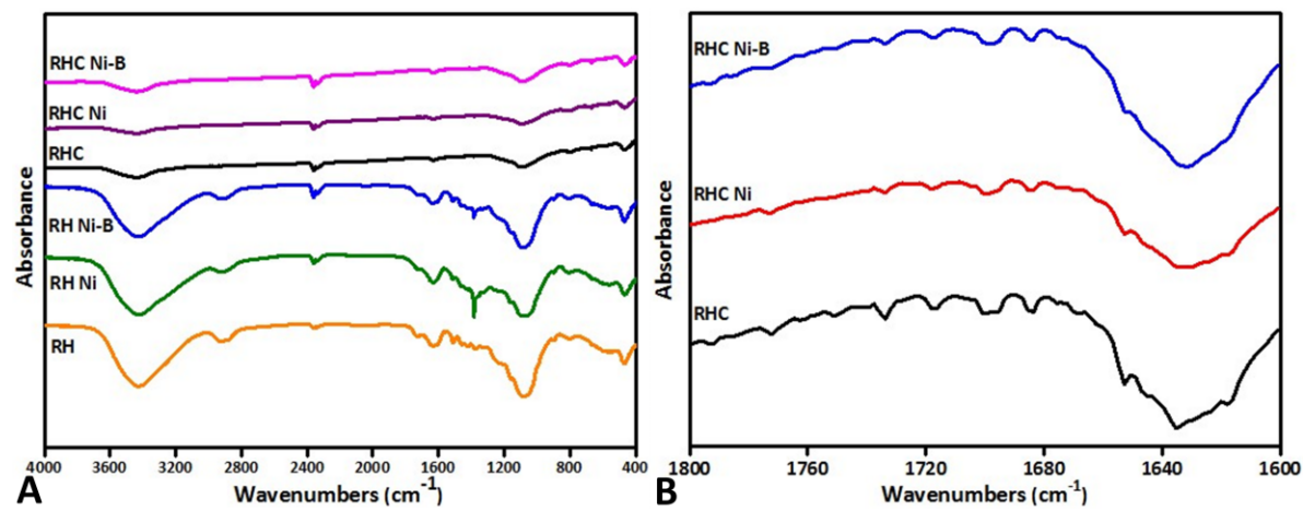
Figure S-3 FTIR spectra of RHs before and after pyrolysis
