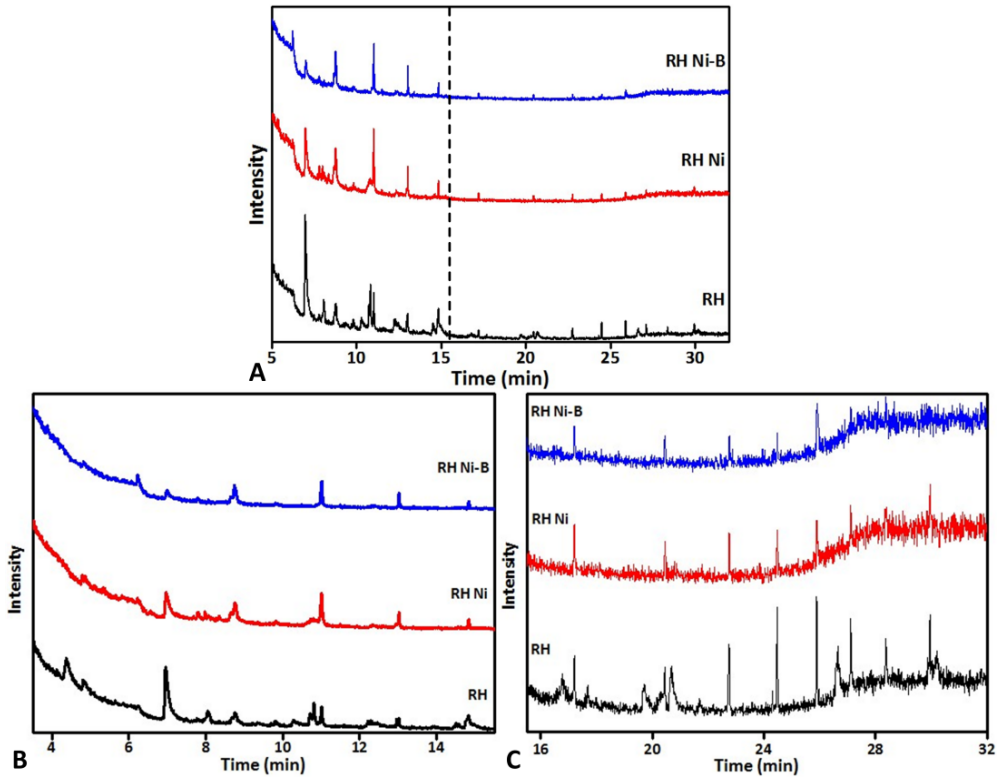
Figure S-2. GC-MS spectra of the collected tar samples
