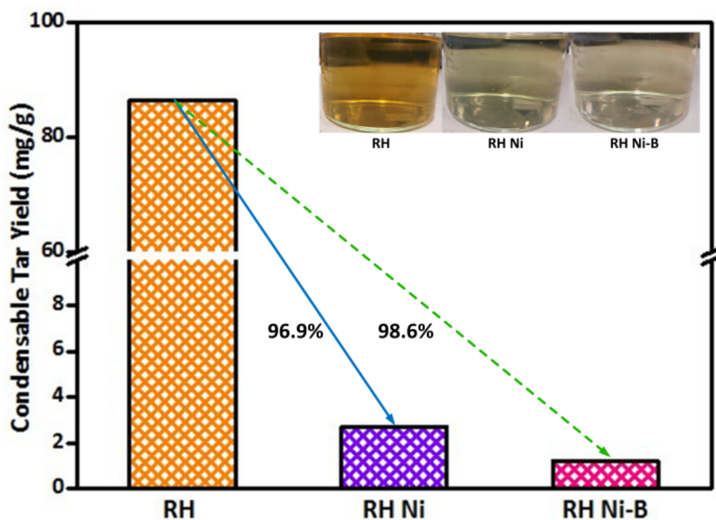
Figure S-1. The condensable tar yields of RHs pyrolysis at 700 °C
