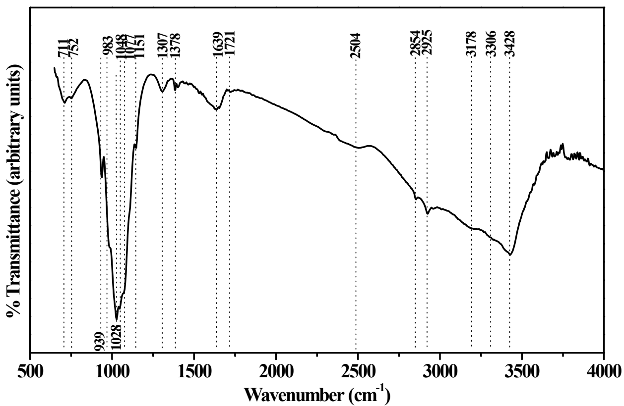
Supplement 2: FT-IR spectrum of manganese phosphate coatings deposited on the mild steel anode at 4 mA/cm 2
