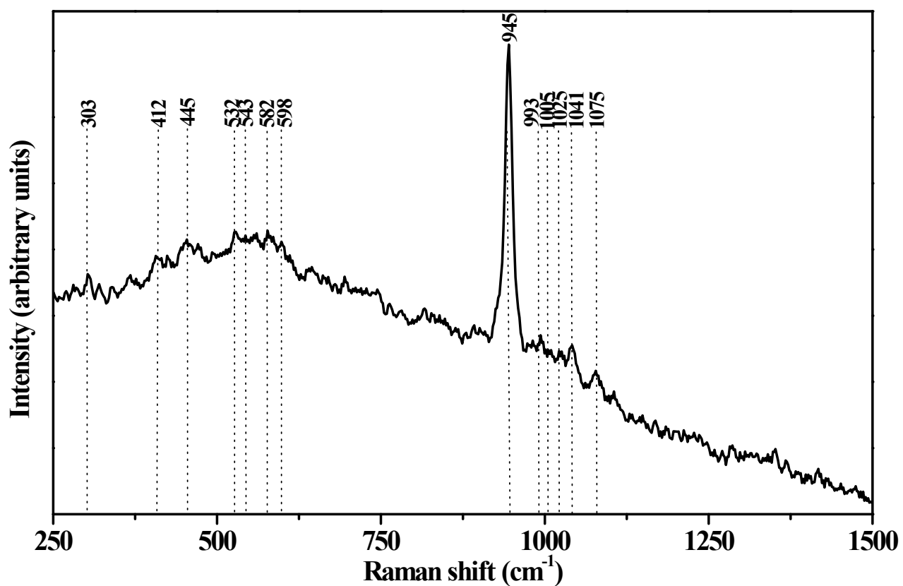
Supplement 3: Raman spectrum of the manganese phosphate coating deposited on the mild steel anode at 4 mA/cm 2
