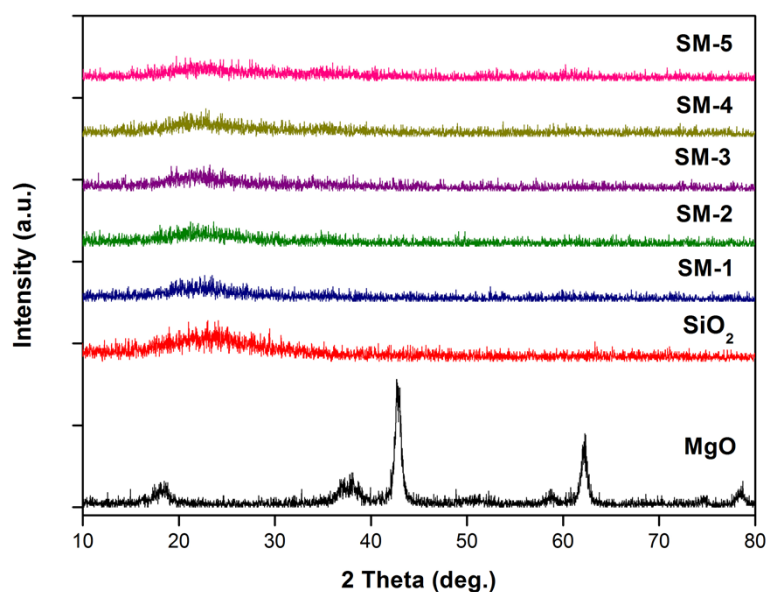
Fig.S1 X-ray diffraction patterns of SM-1 to SM-5 with different magnesium oxide addition.
