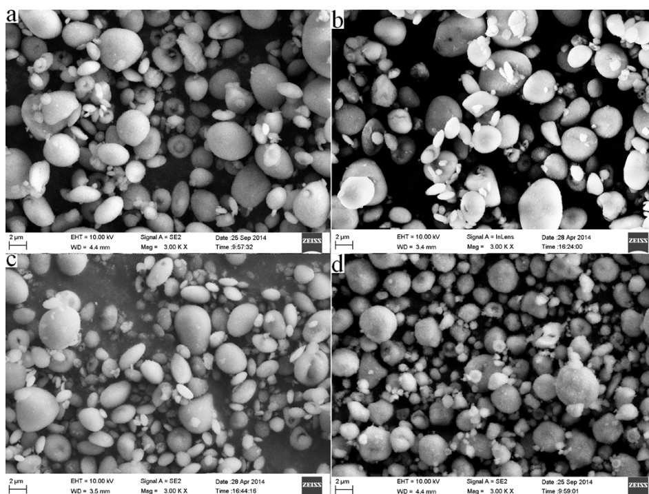
Fig.S2 SEM images of (a) SM-1; (b) SM-2; (c) SM-3; (d) SM-4.
