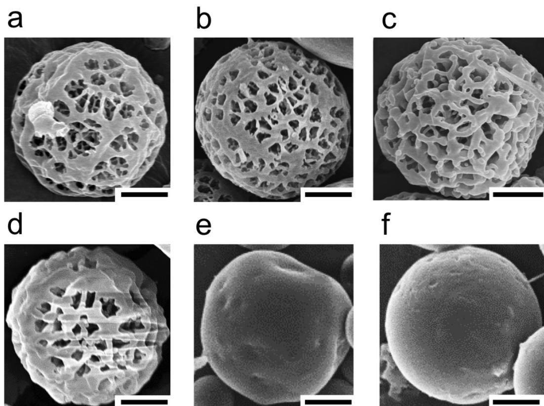
Figure S1. SEM photographs of the prepared PMMA microspheres prepared using different volumes of DCM were used: 3 mL (a), 4 mL (b), 5 mL (c), 6 mL (d), 7 mL (e), and 8 mL (f). Scale bar = 5 \mu\text{m} .
