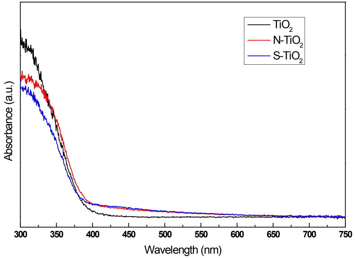
Fig. 2. UV-vis spectra of TiO 2 , N-TiO 2 and S-TiO 2 annealed at 450°C in Ar atmosphere.
