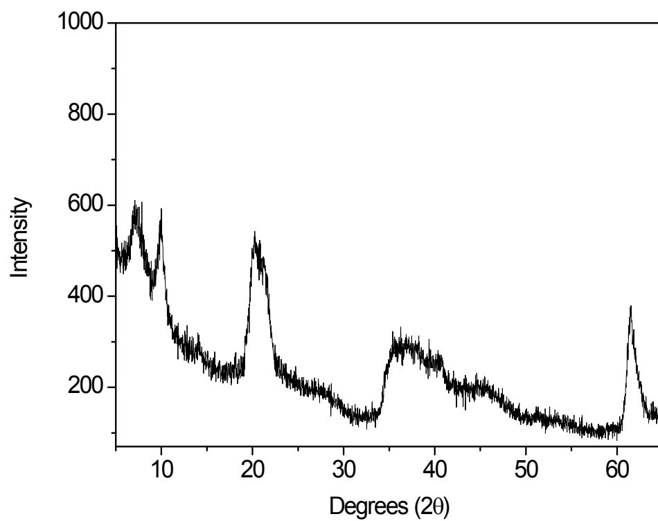
SI 4. PXRD pattern of Mg/Al-CH 3 COO LDH restacked without freeze drying.
