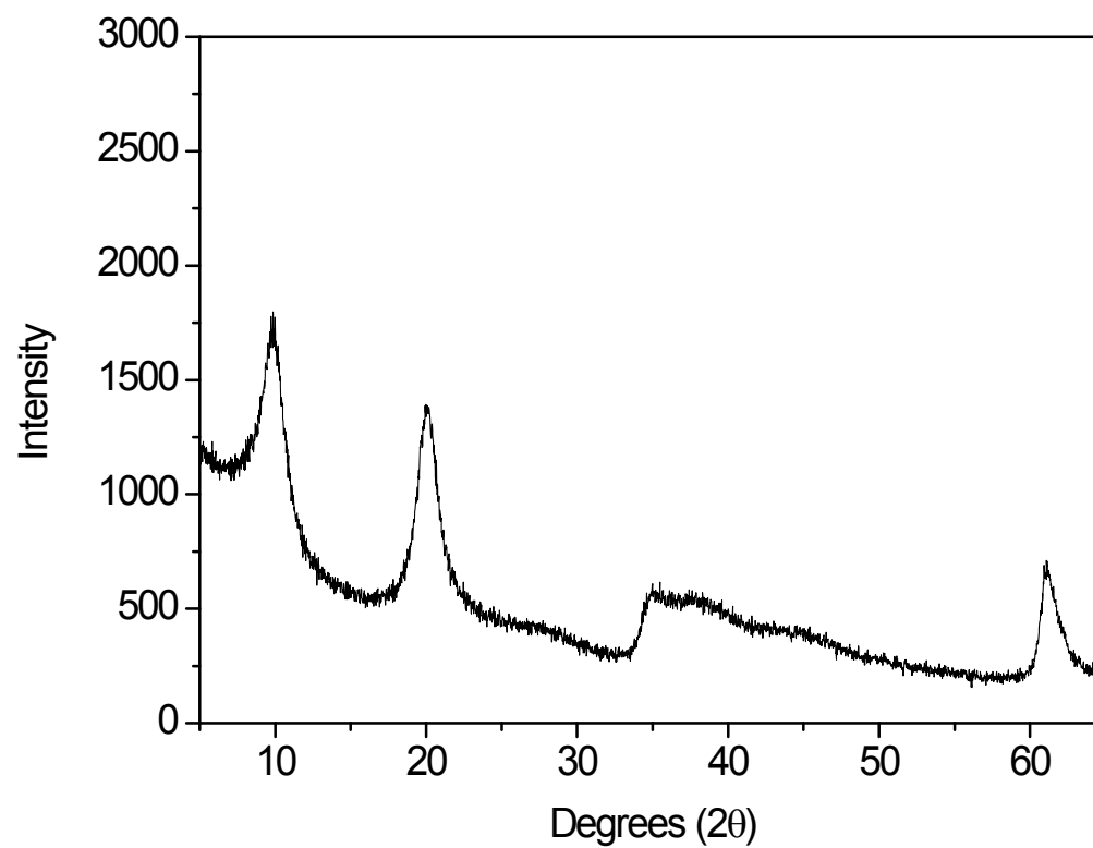
SI 1. PXRD pattern of Mg/Al-NO 3 LDH prepared from ammonia precipitation.
