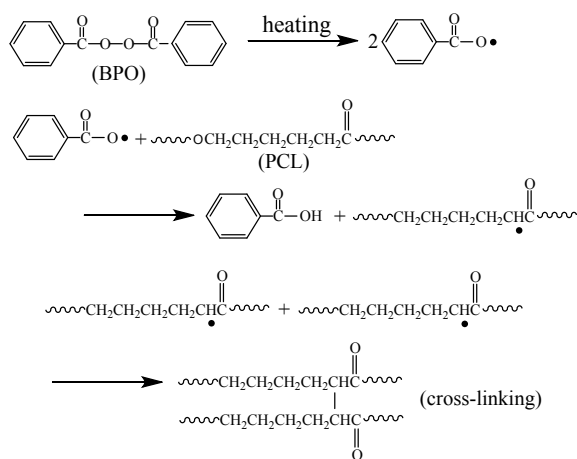
Fig.S1 The scheme of cross-linking reactions between PCL and BPO.
