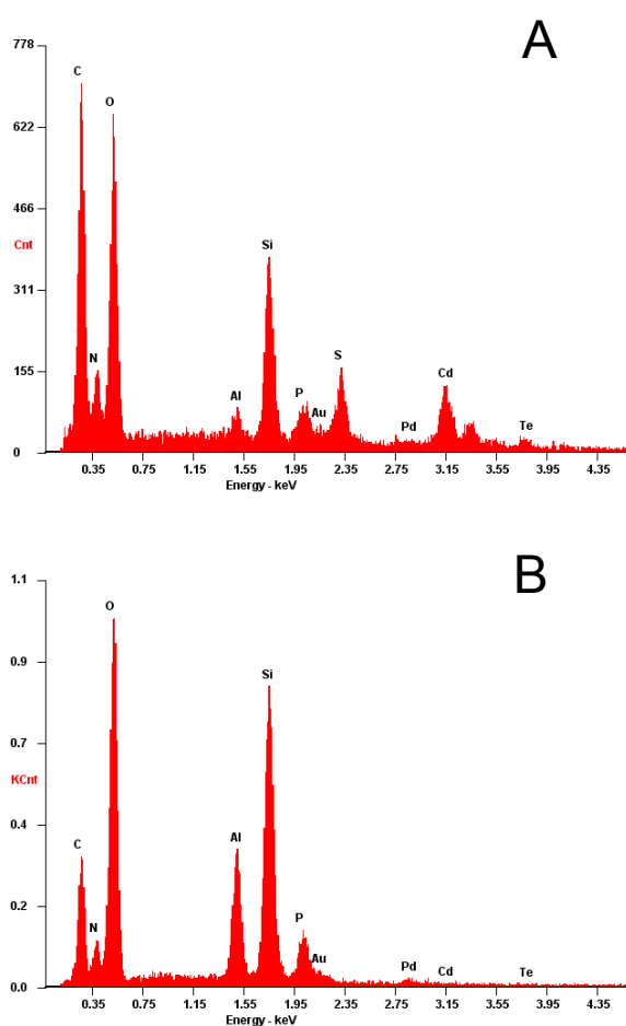
Fig. 1. Elemental analysis, of synthesized nanoparticles with (A) and without (B) encapsulated QDs, by electron diffraction x-ray spectroscopy (EDS).
