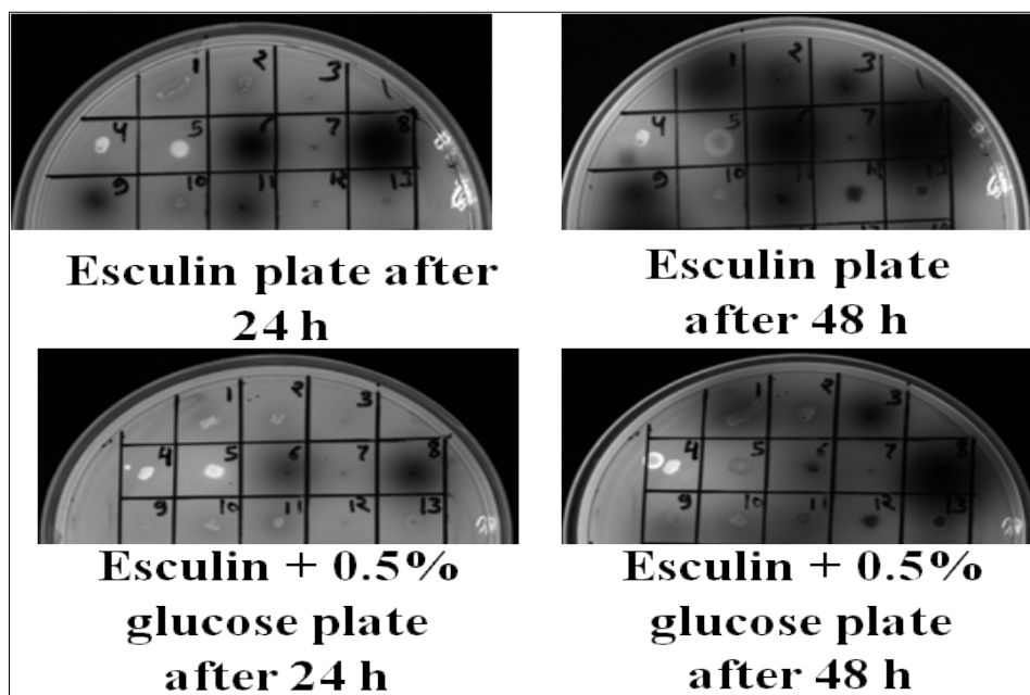
ESI Fig.1. Qualitative screening of \beta -glucosidase activity on agar medium containing esculin with or without glucose
