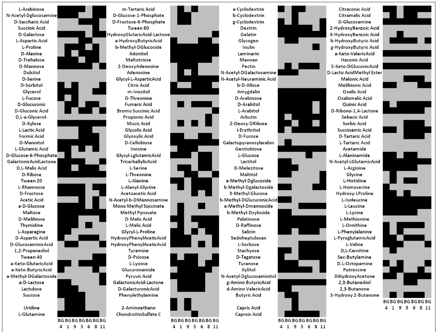
ESI Fig.2. Carbon source usage of selected isolates via BIOLOG PM assays plates. Black and gray boxes represent usage or no usage of carbon substrate, respectively
