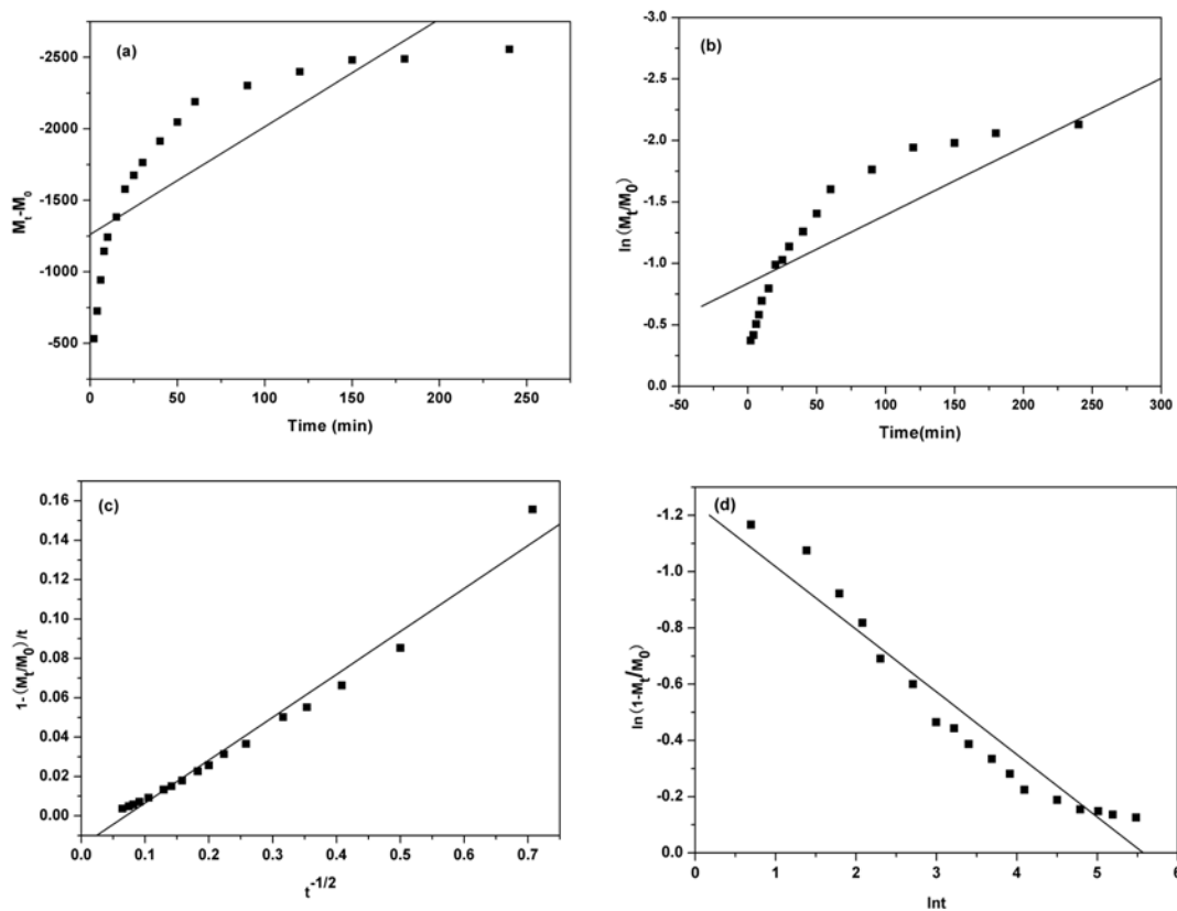
Fig.S1. Plots of four different kinetic models for the release of dexa from Dexa-LDHs at pH=7.4
