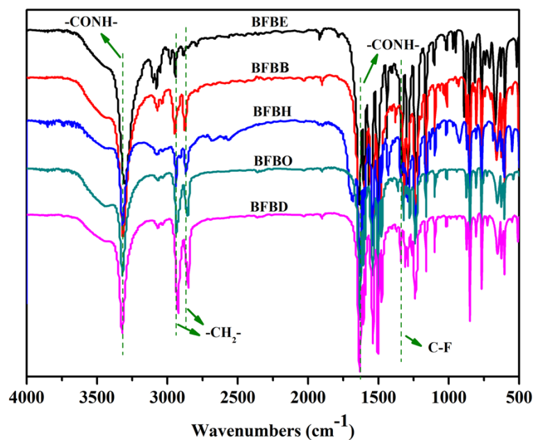
Supplementary data Figure 1 The FT-IR spectra of monomers (BFBE, BFBB, BFBH, BFBO, BFBD).
