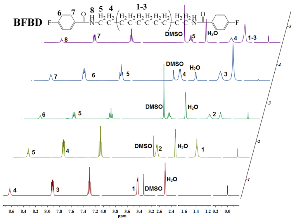
Supplementary data Figure 2 The ^1\text{H-NMR} spectra of monomers (BFBE, BFBB, BFBH, BFBO, BFBD).
