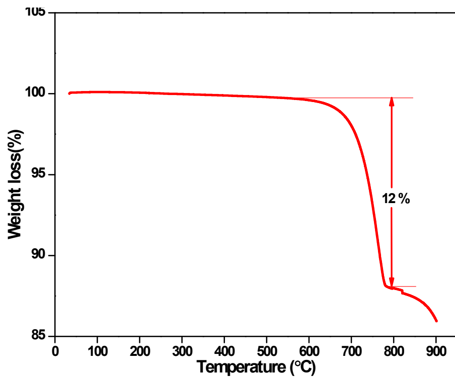
Fig. S1. TGA curve of BiOCl compound.
