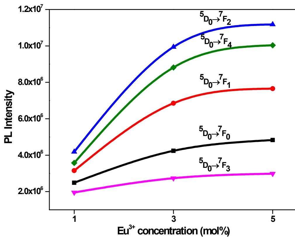
Fig. S3. Variation in the PL intensity with different transitions as a function of the \text{Eu}^{3+} ion concentration in \text{BiOCl} .
