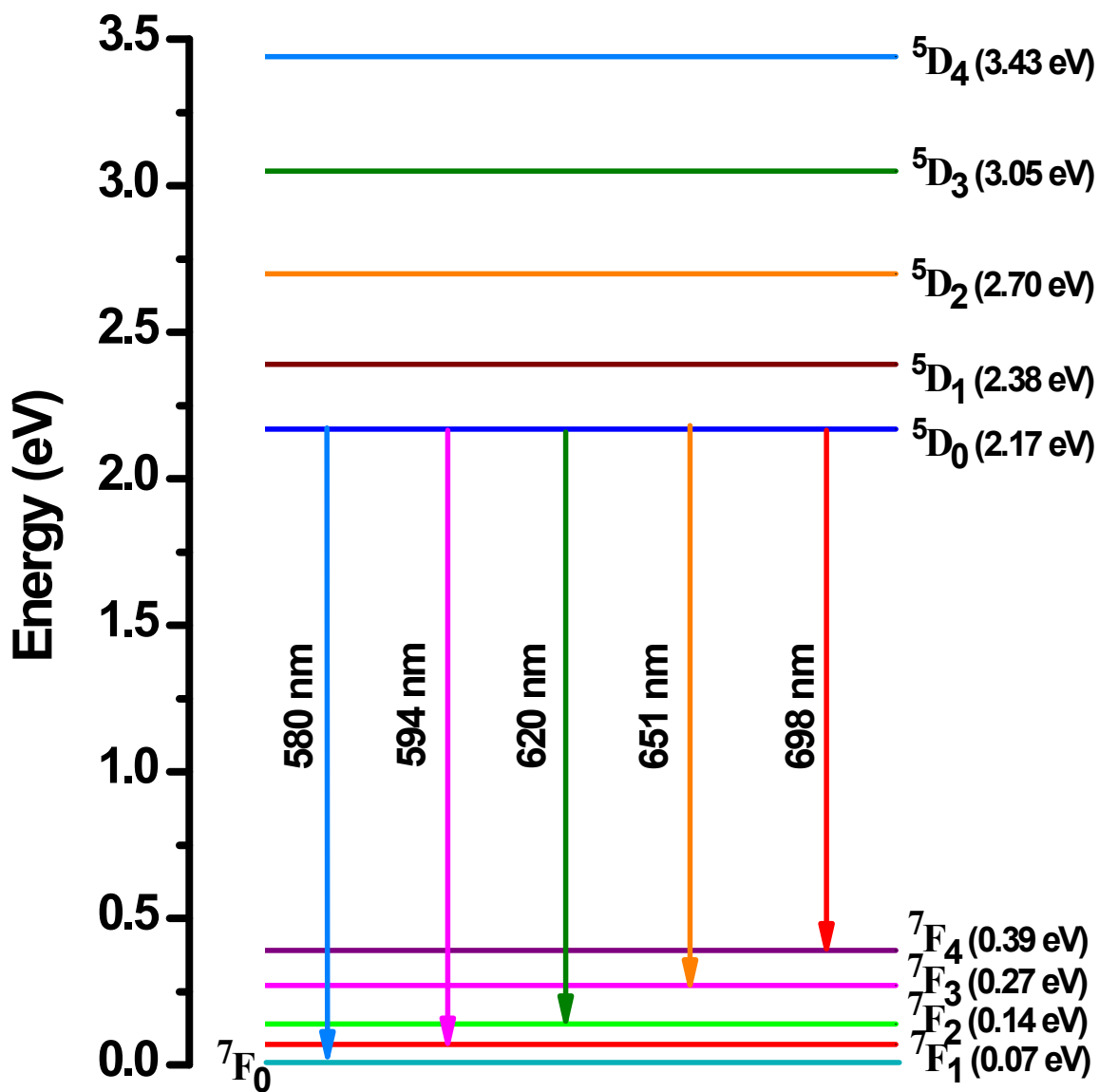
Fig. S2. Energy level diagram for \text{Eu}^{3+} ion in \text{Bi}_{1-x}\text{Eu}_x\text{OCl} phosphors.
