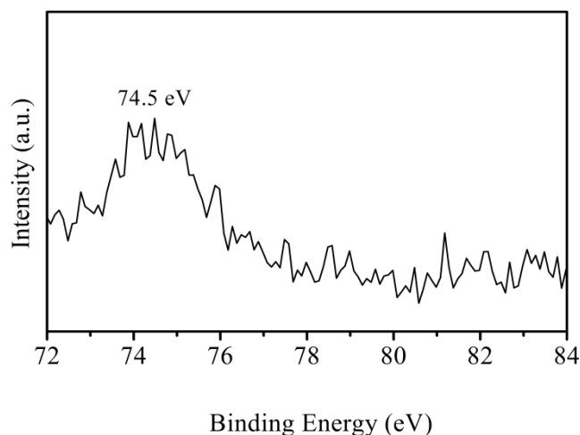
Fig. S1. XPS survey patterns of the binding energy for Al 2p electrons on the surface of Ni/Al 2 O 3 composites.
