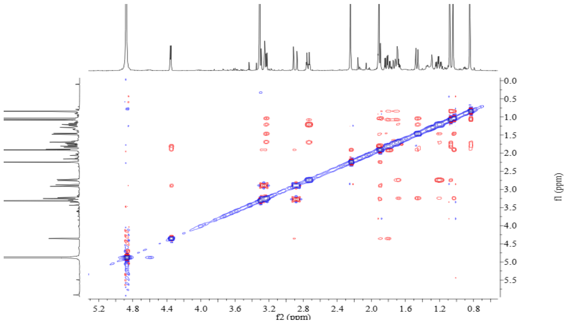
Lanceolatin C (3)
