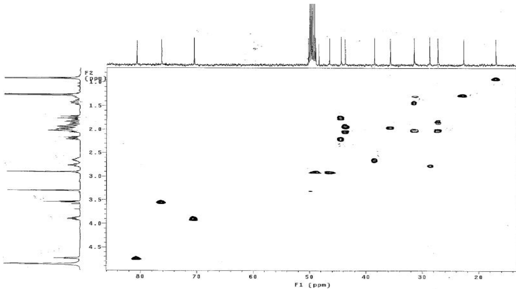
Figure S53 HMBC of Lanceolatin G (7)
