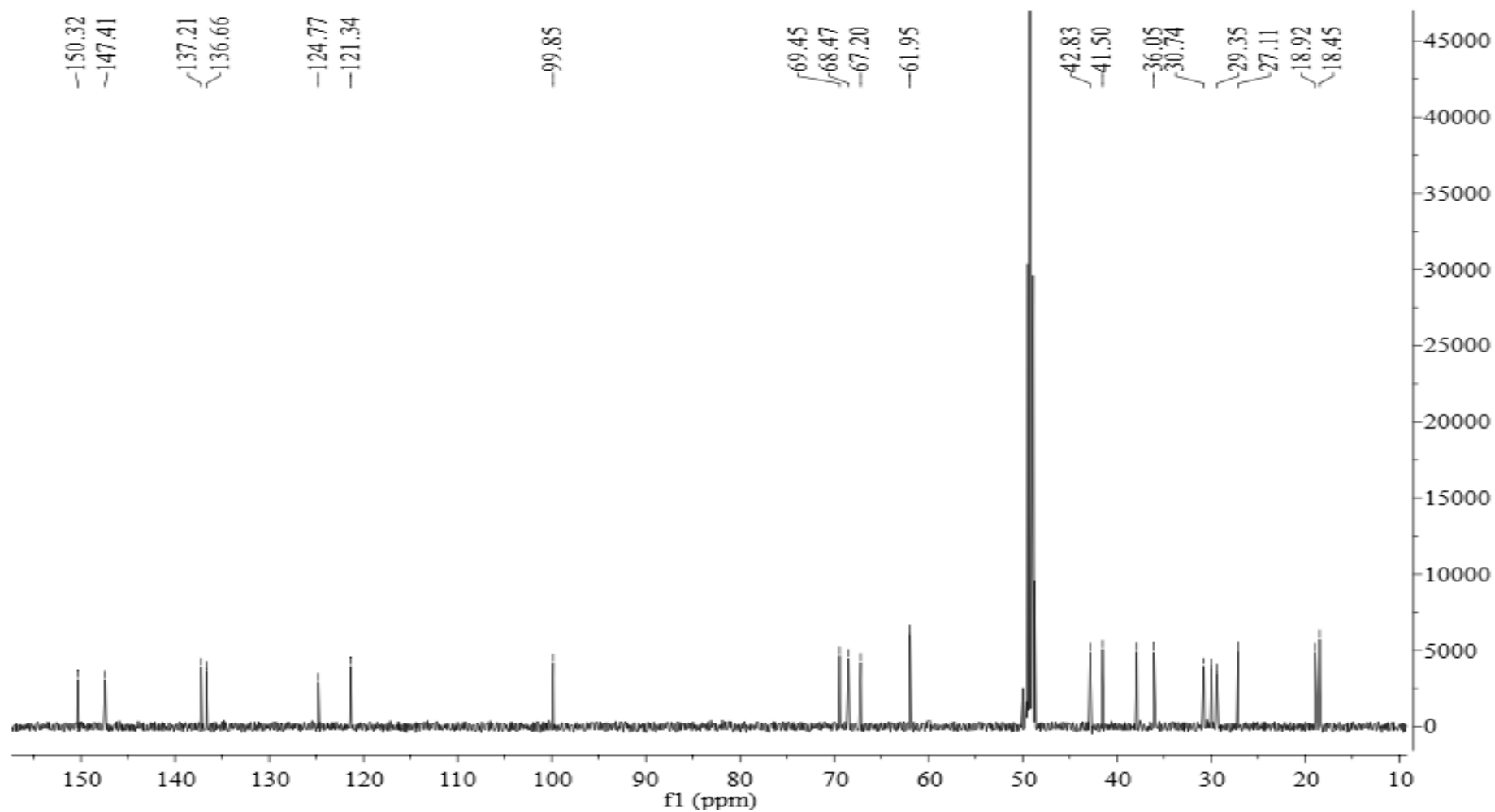
Figure S36 DEPT of Lanceolatin E (5)
