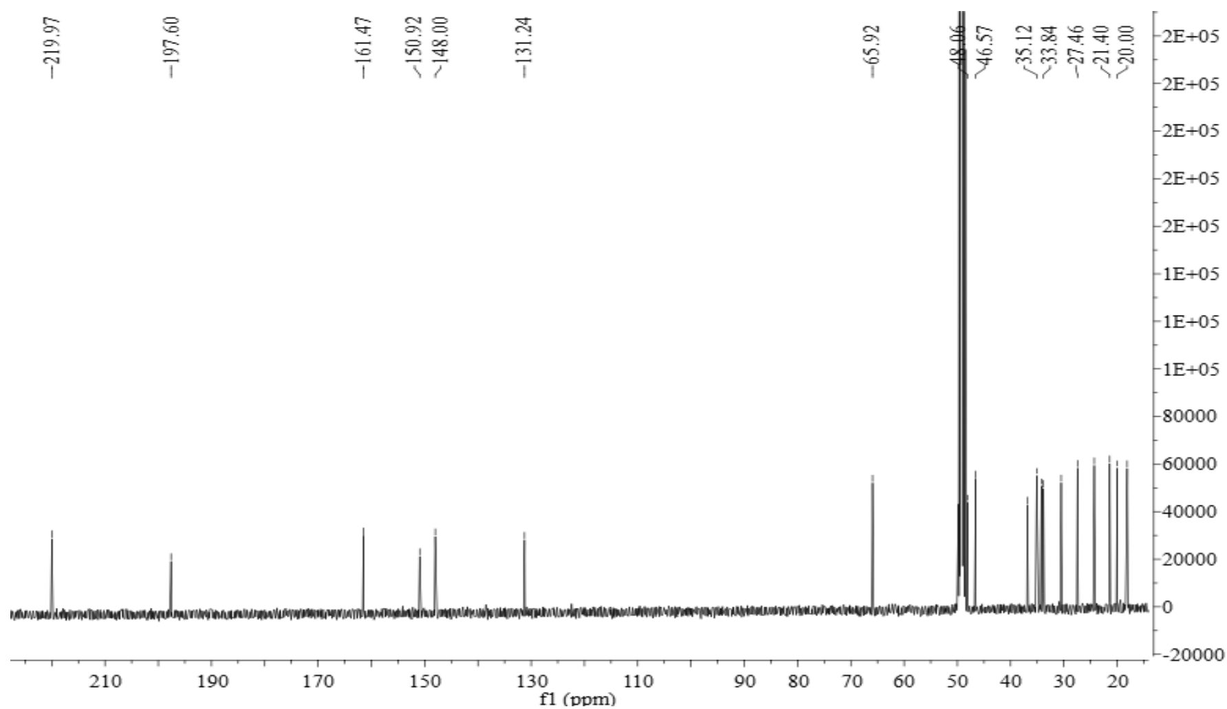
Figure S21 DEPT of Lanceolatin C (3)
