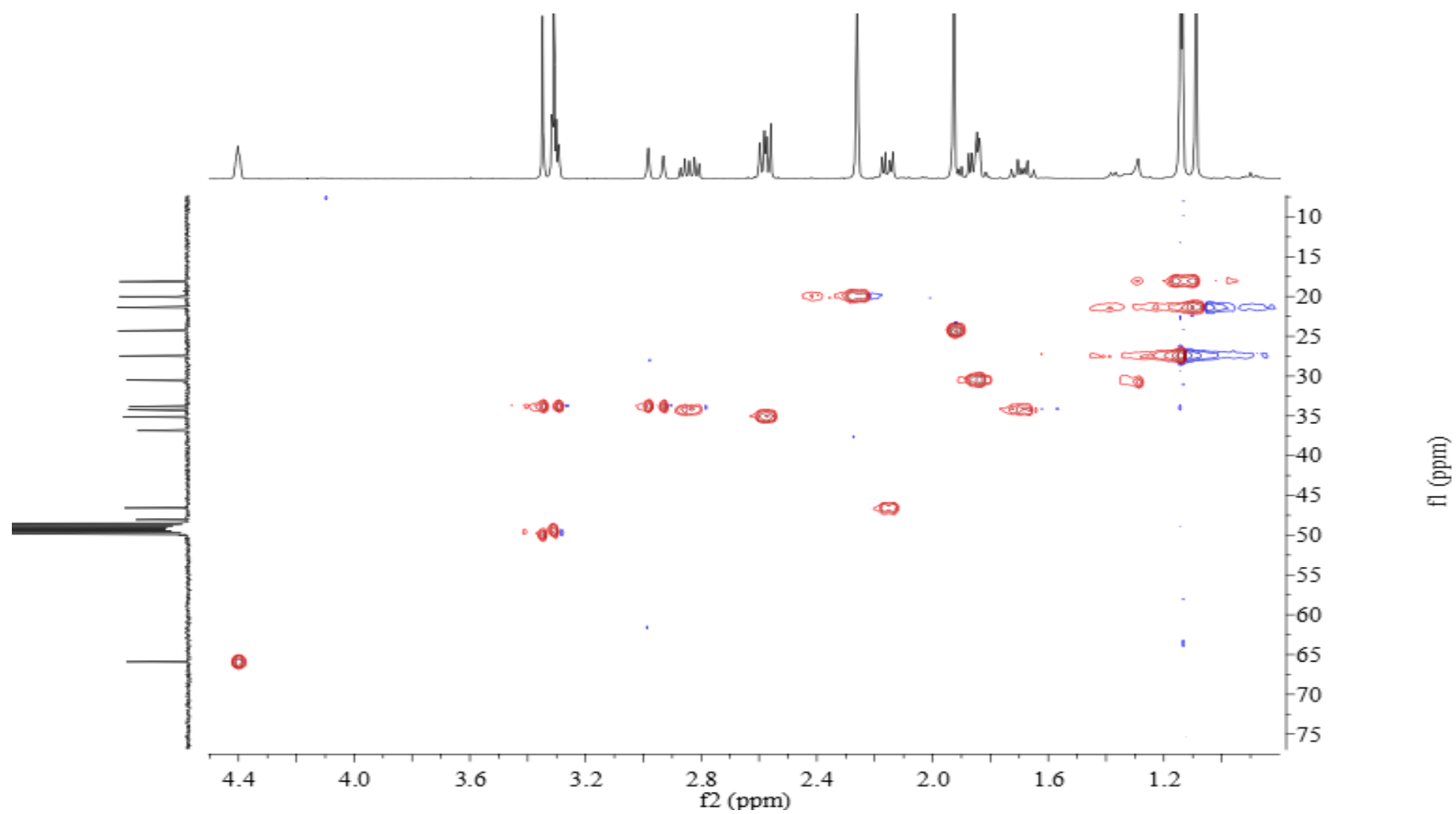
Figure S23 HMBC of Lanceolatin C ( 3 )
