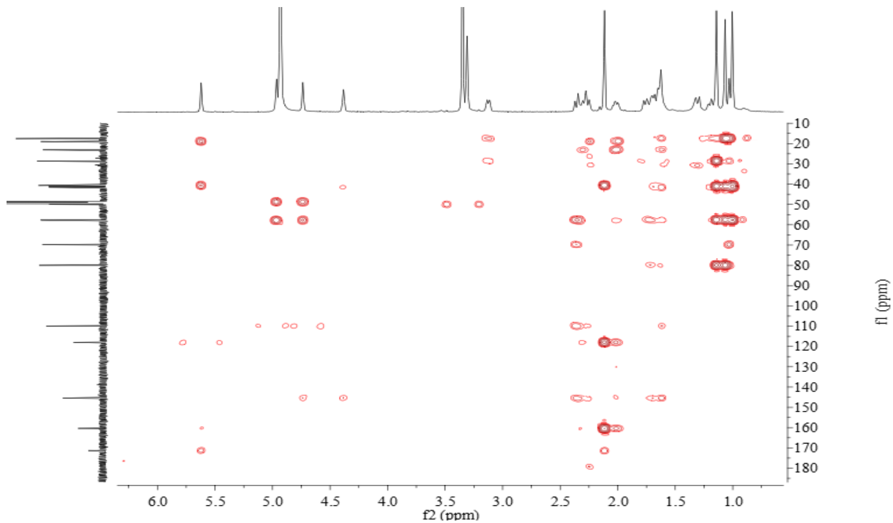
Figure S7 HMBC of Lanceolatin A ( 1 )
