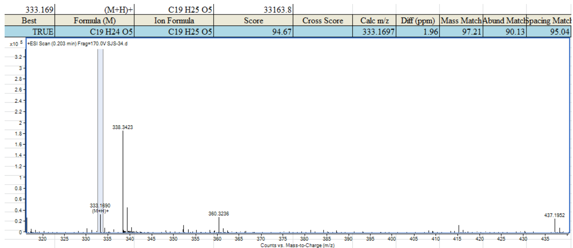
Figure S48 HR-ESI-MS of Lanceolatin G (7)
