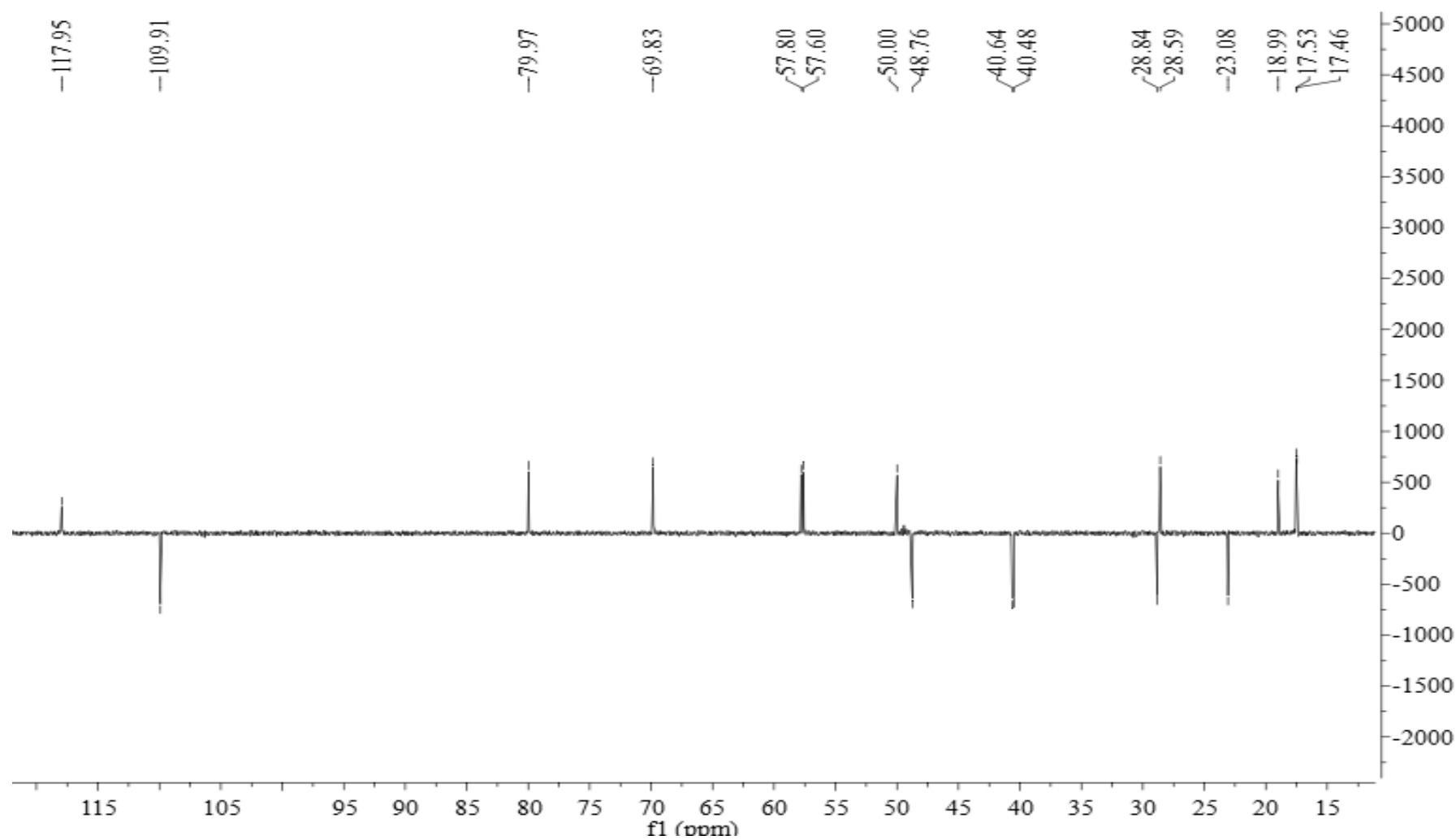
Figure S5 DEPT of Lanceolatin A ( 1 )
