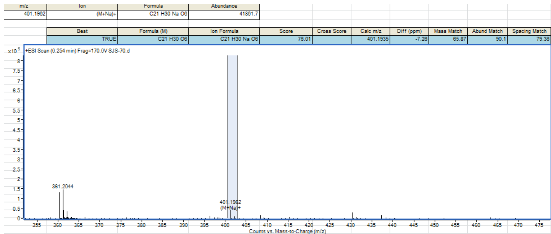
Figure S40 HR-ESI-MS of Lanceolatin F
