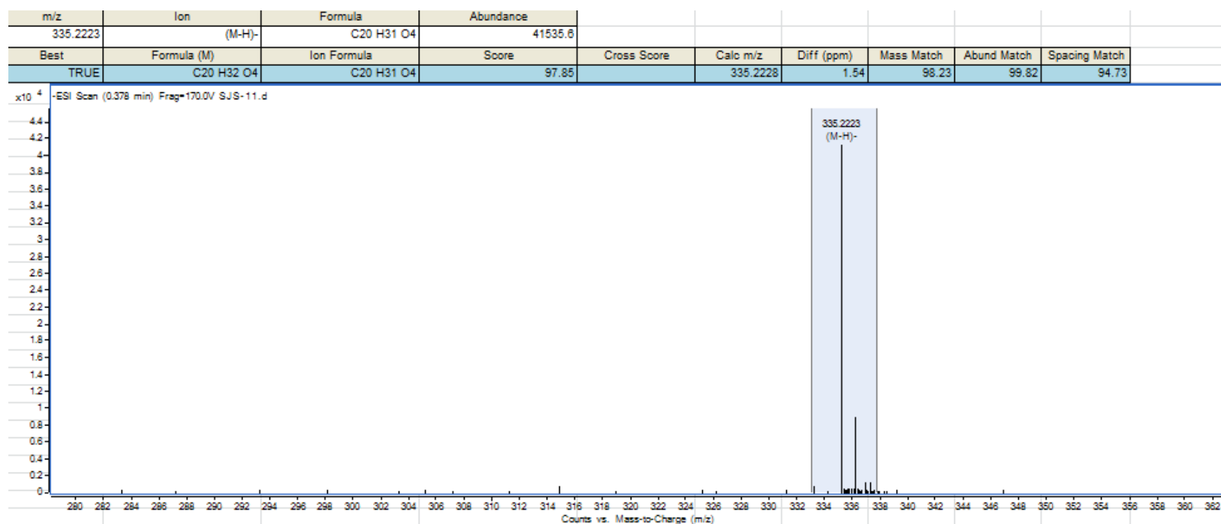
Figure S1 HR-ESI-MS of Lanceolatin A (1)
