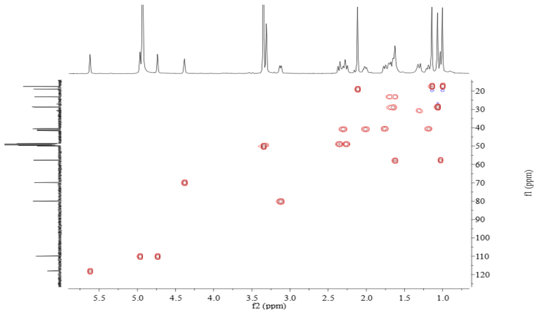
Figure S6 HMQC of Lanceolatin A ( 1 )
