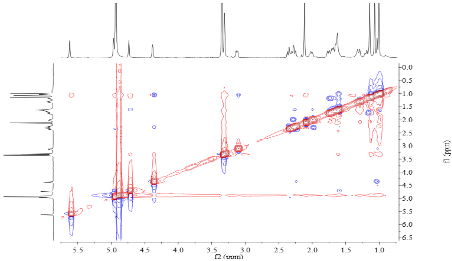
Figure S8 NOSEY of Lanceolatin A ( 1 )
