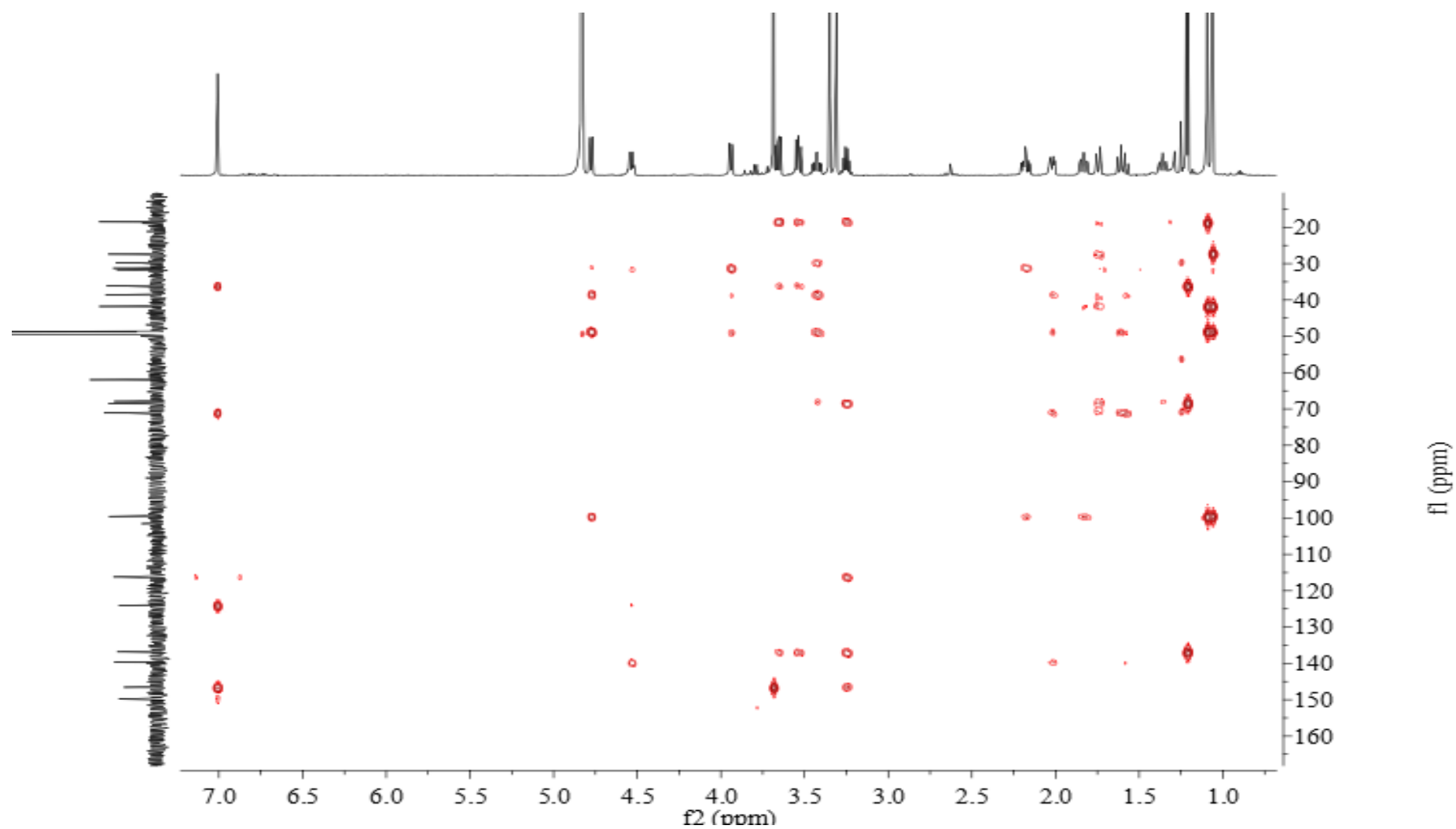
Figure S47 NOSEY of Lanceolatin F ( 6 )
