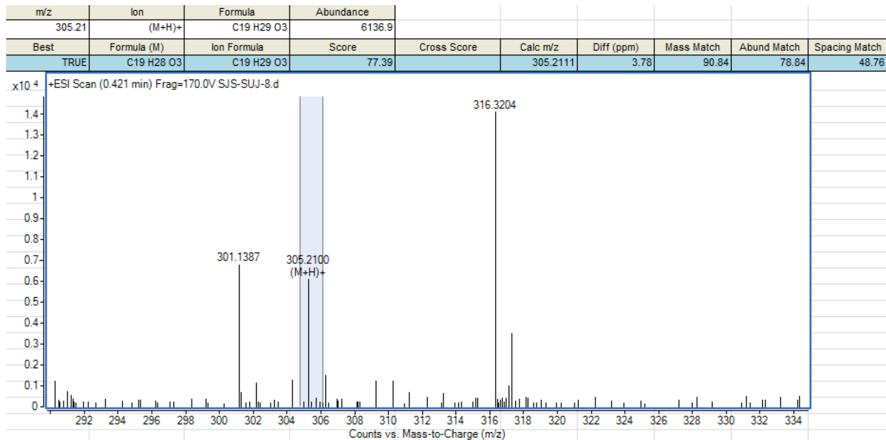
Figure S9 HR-ESI-MS of Lanceolatin B
