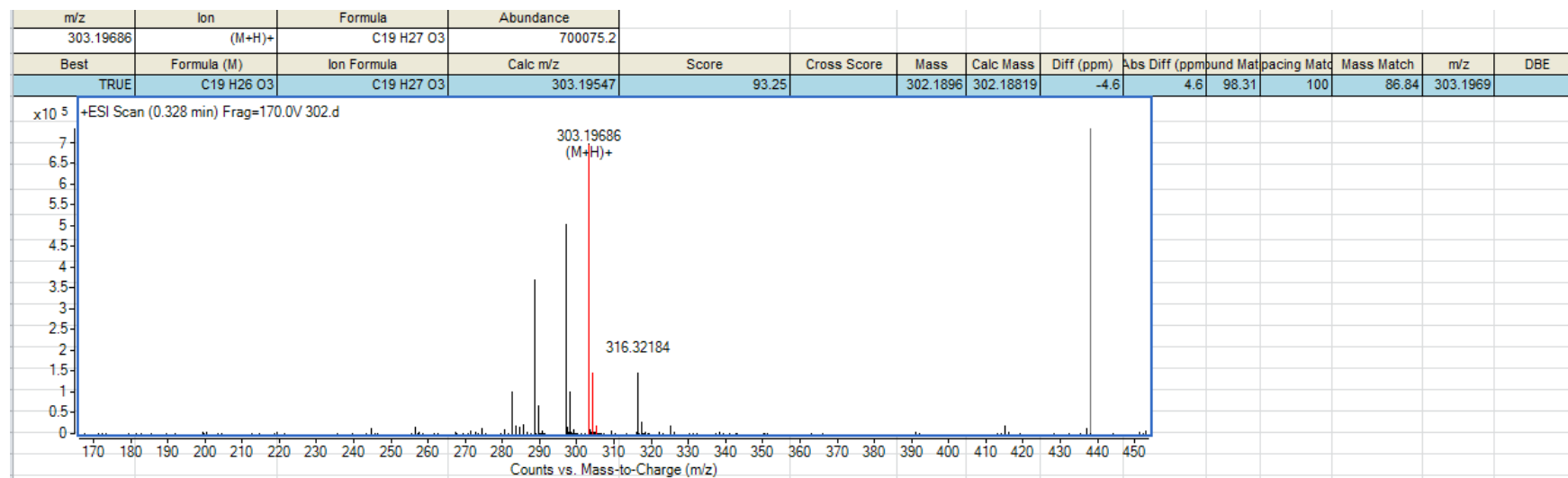
Figure S17 HR-ESI-MS of Lanceolatin C
