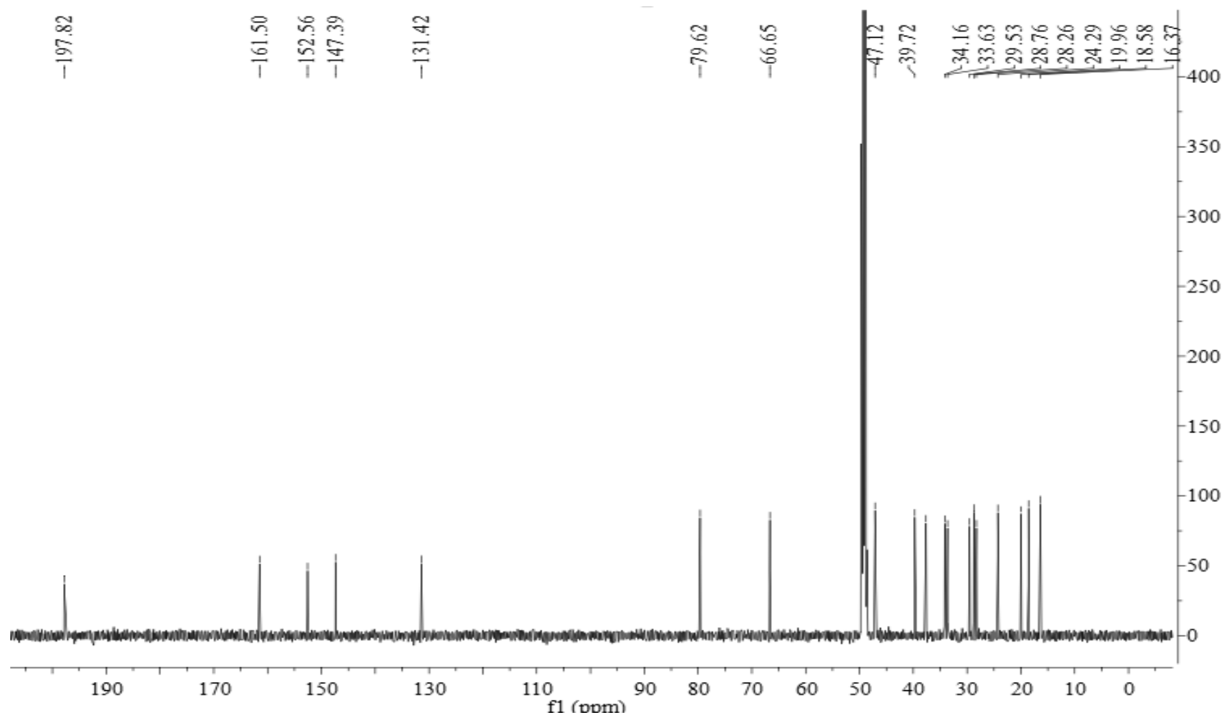
Figure S13 DEPT of Lanceolatin B (2)
