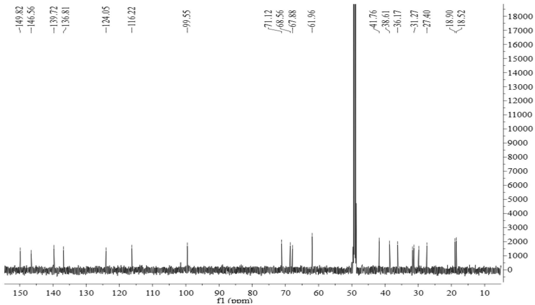
Figure S44 DEPT of Lanceolatin F (6)
