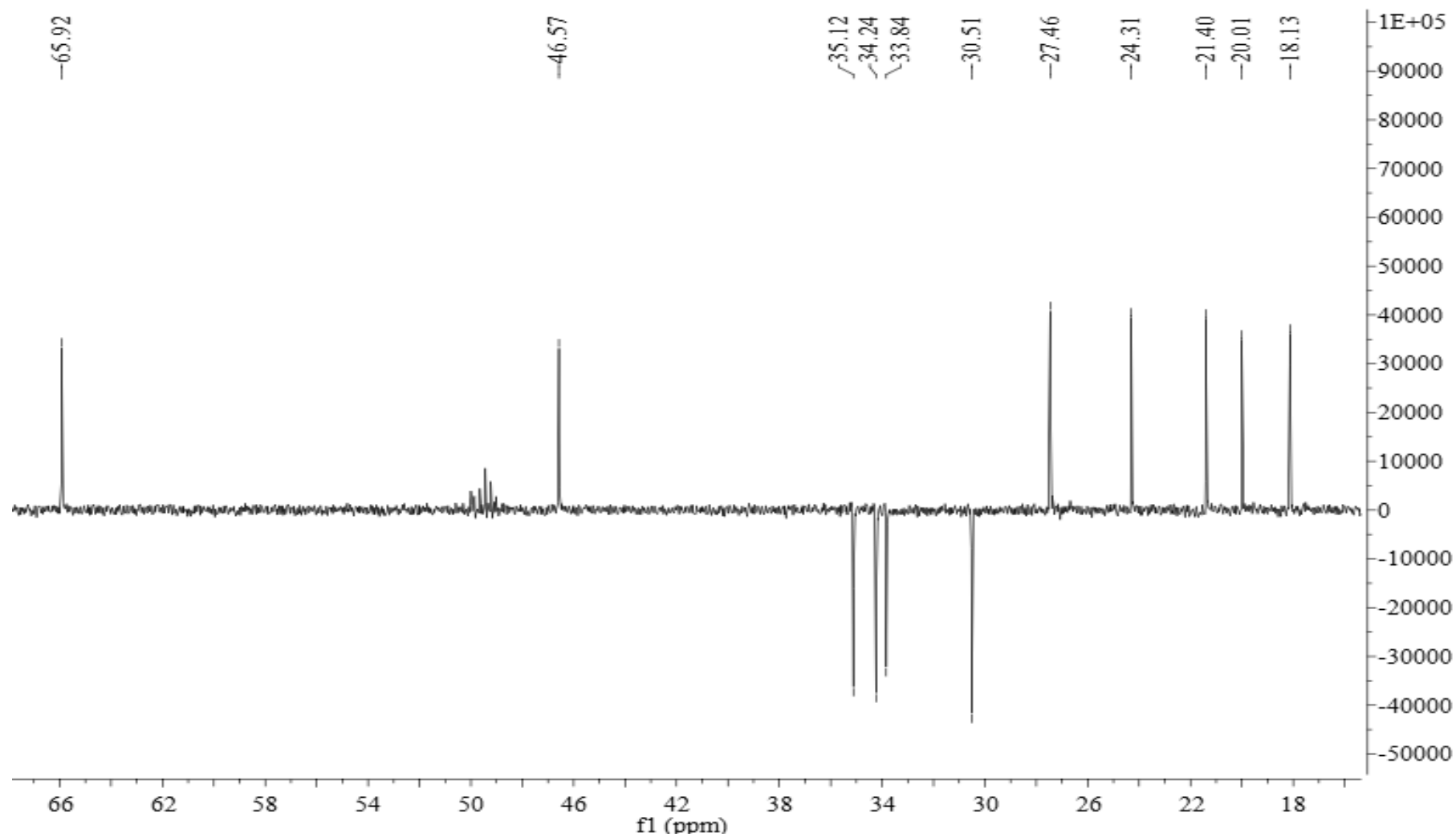
Figure S22 HMQC of Lanceolatin C (3)
