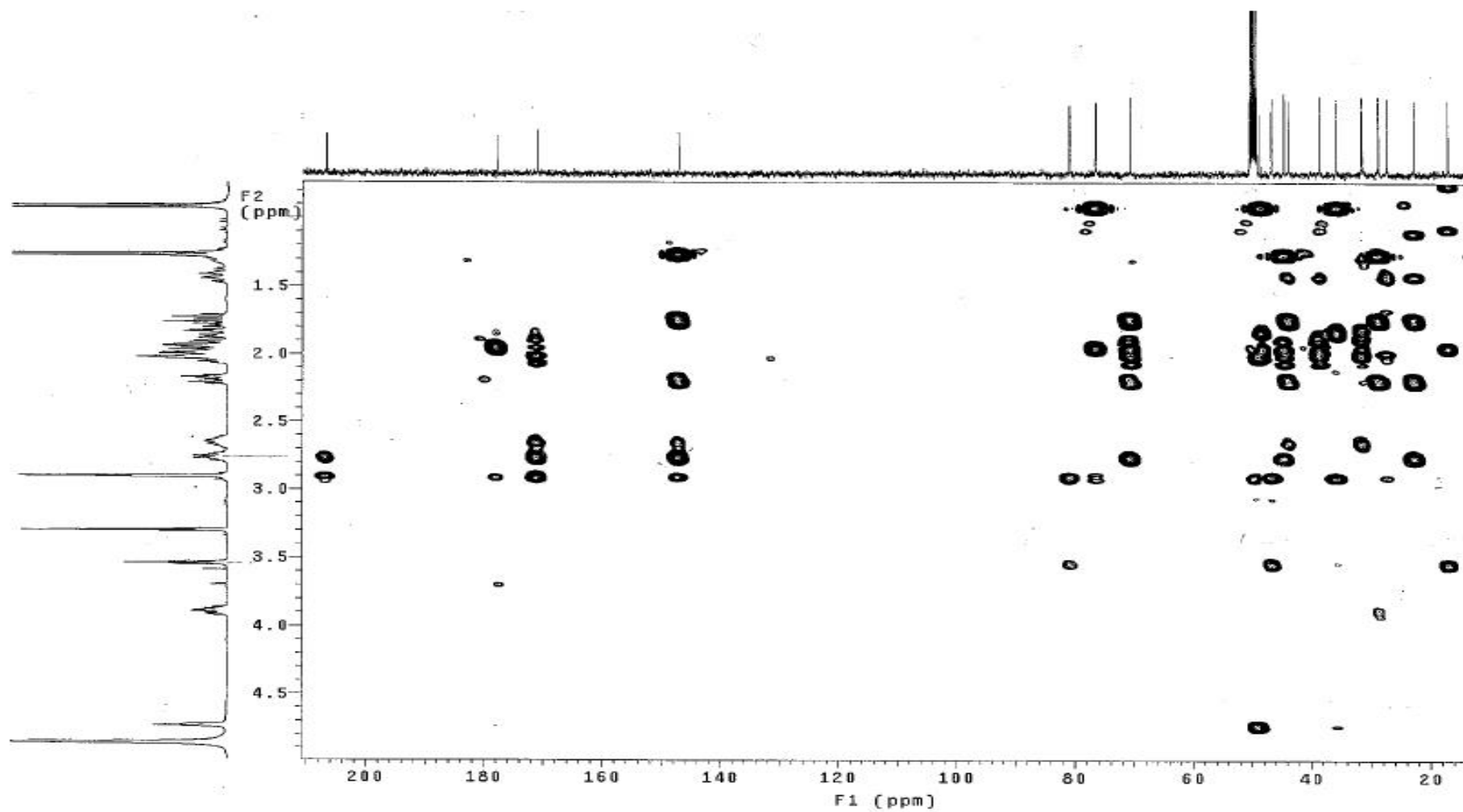
Figure S54 NOSEY of Lanceolatin G (7)
