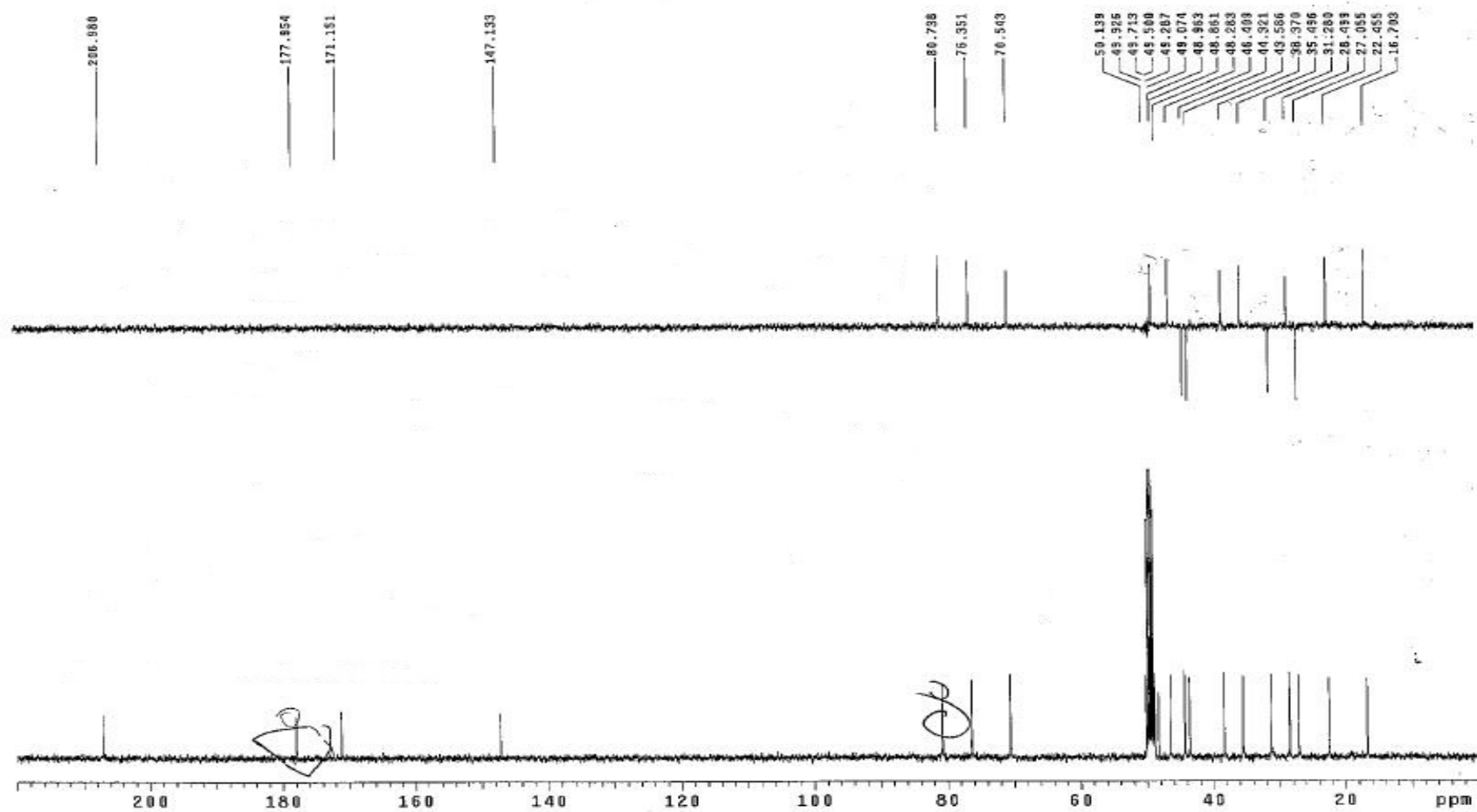
Figure S52 HMQC of Lanceolatin G (7)
