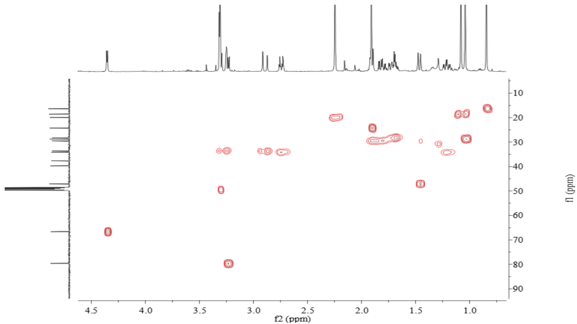
Figure S15 HMBC of Lanceolatin B ( 2 )
