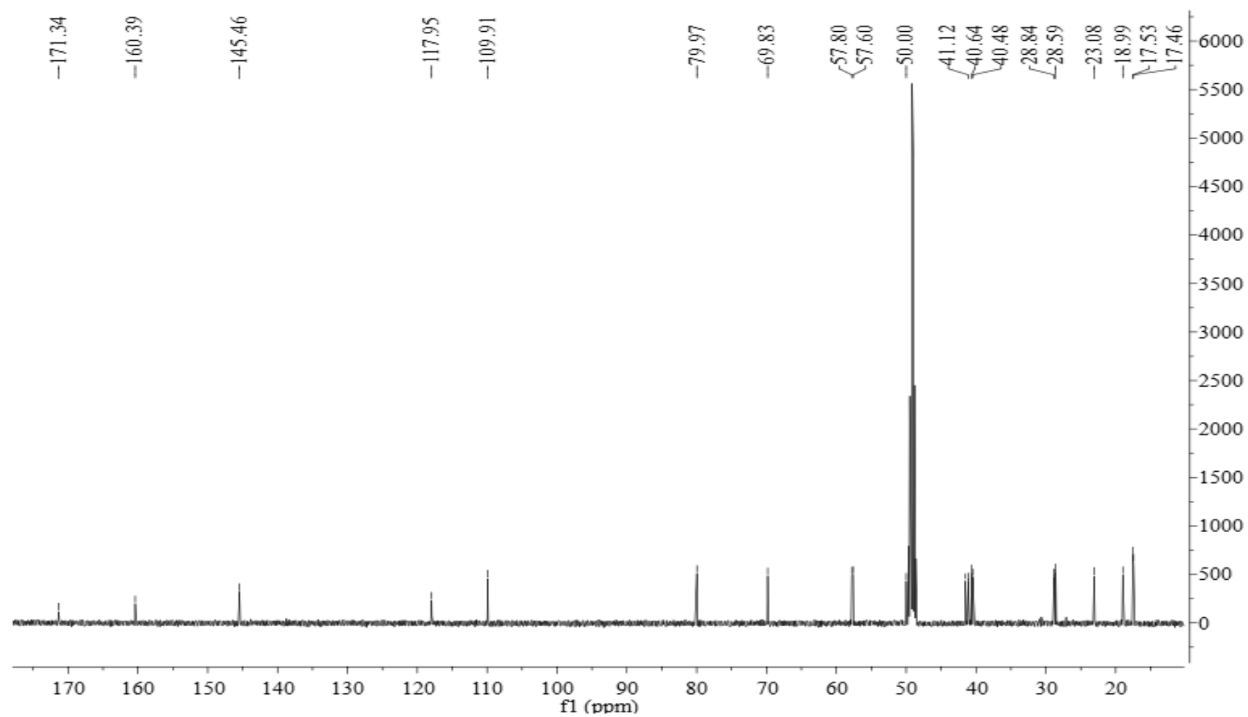
Figure S4 ^{13}\text{C} NMR of Lanceolatin A ( 1 )
