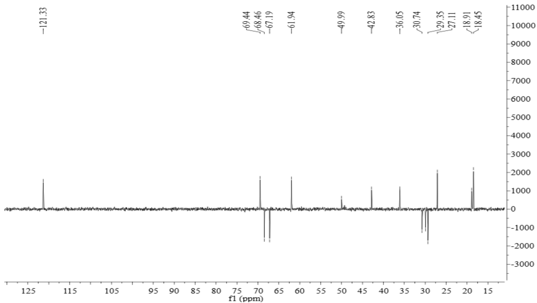
Figure S37 HMQC of Lanceolatin E (5)
