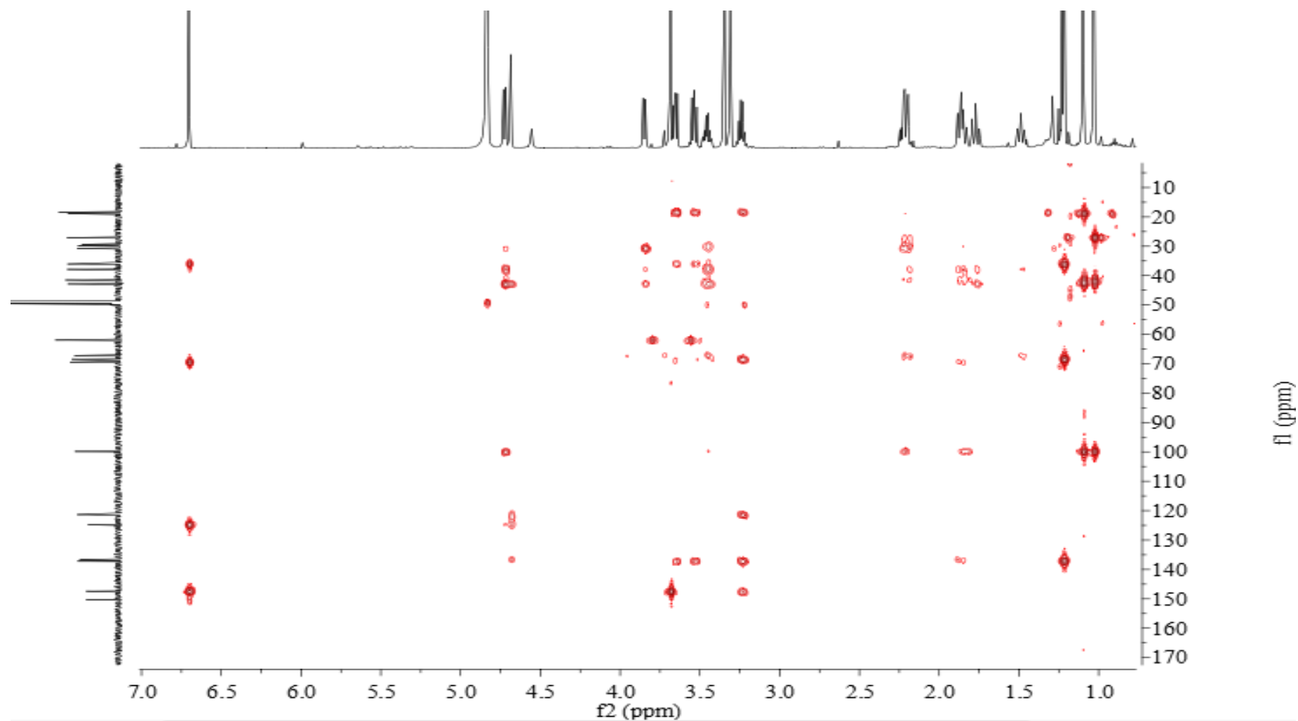
Figure S39 NOSEY of Lanceolatin E (5)
