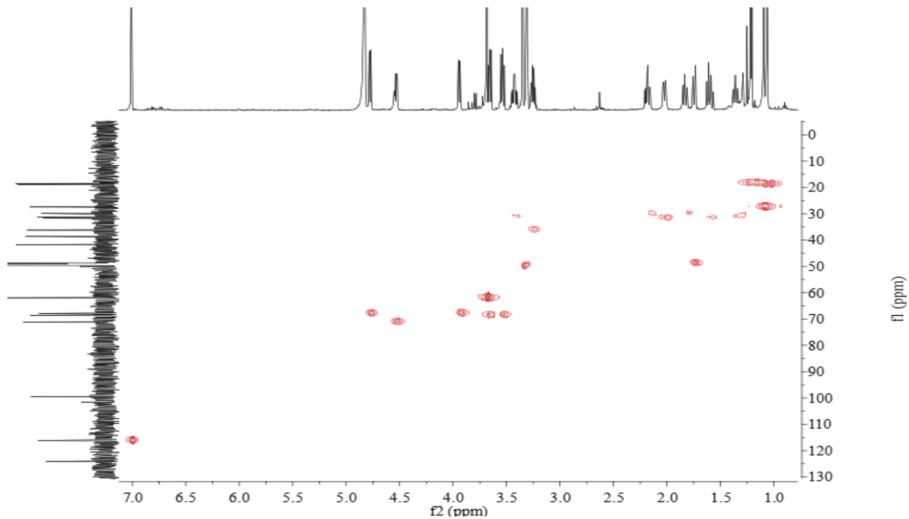
Figure S46 HMBC of Lanceolatin F ( 6 )
