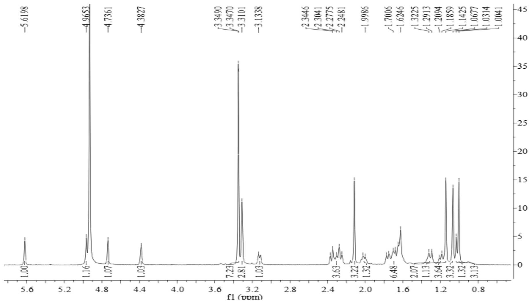
Figure S3 ^1\text{H} NMR of Lanceolatin A ( 1 )
