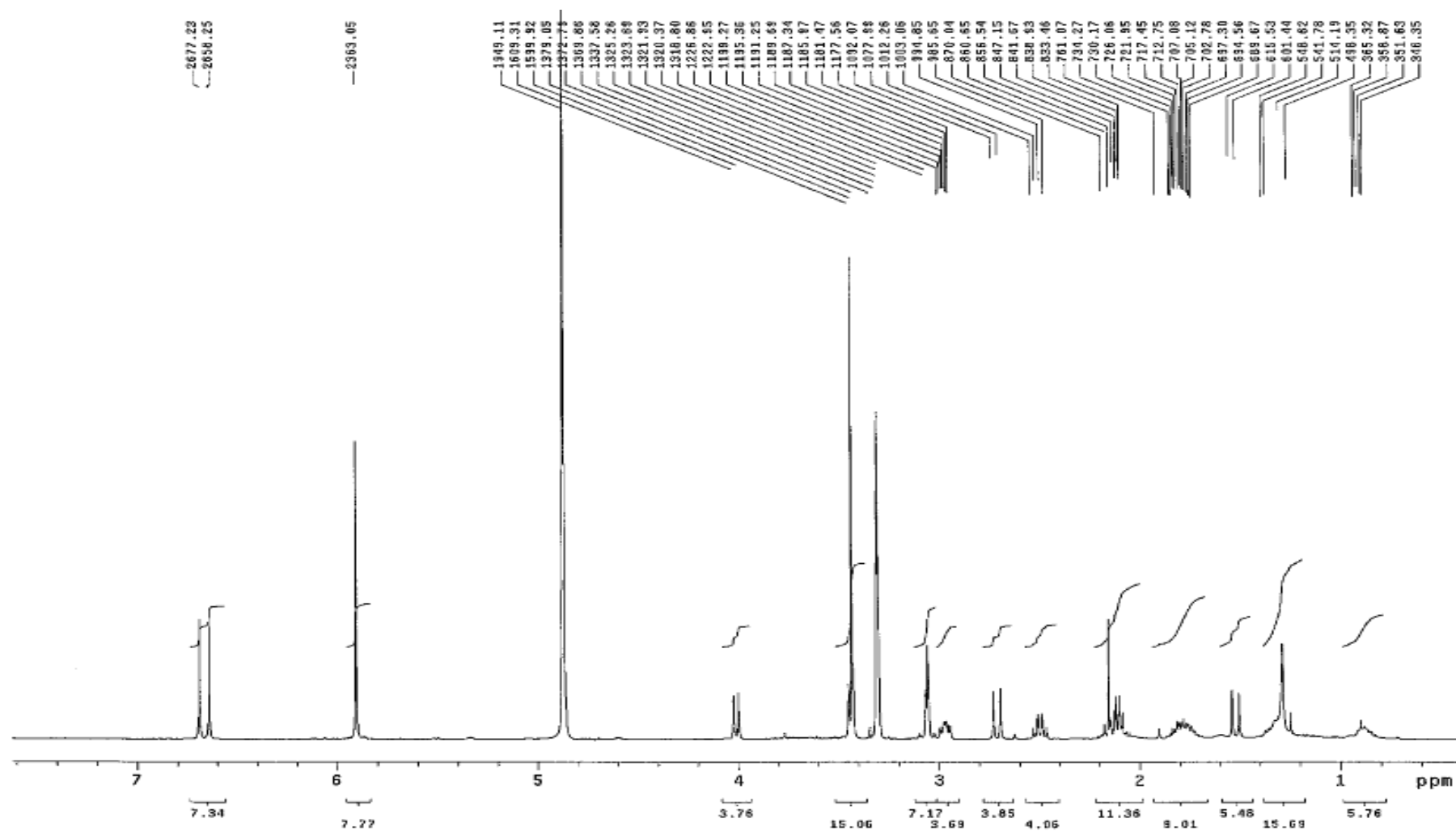
Figure S51 ^{13}\text{C} NMR and DEPT of Lanceolatin G (7)
