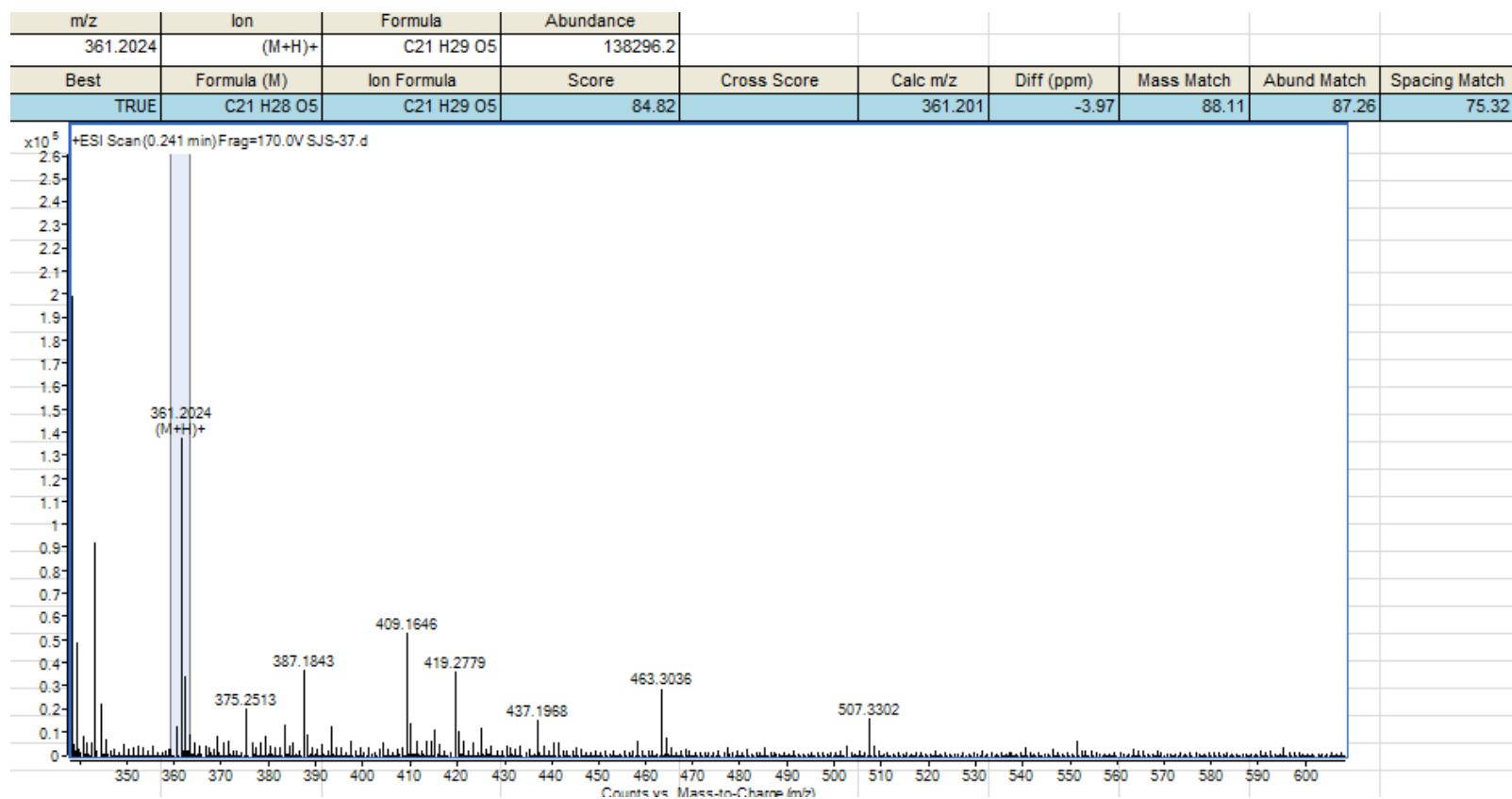
Figure S25 HR-ESI-MS of Lanceolatin D
