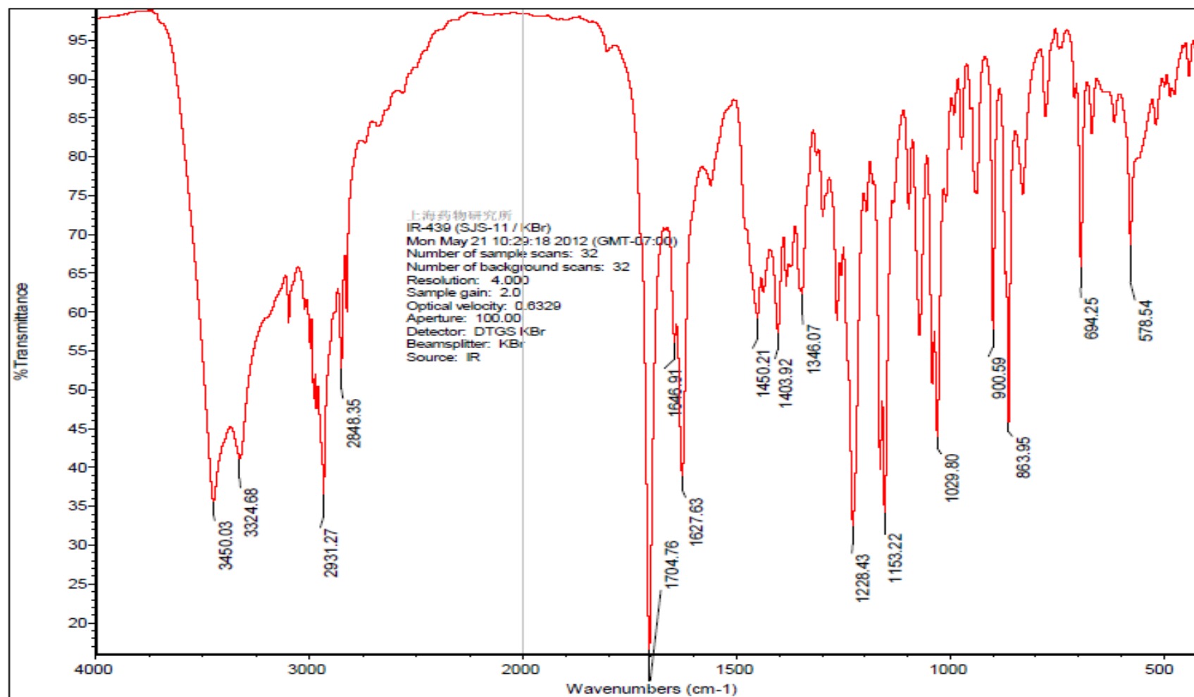
Figure S2 IR(KBr) of Lanceolatin A ( 1 )
