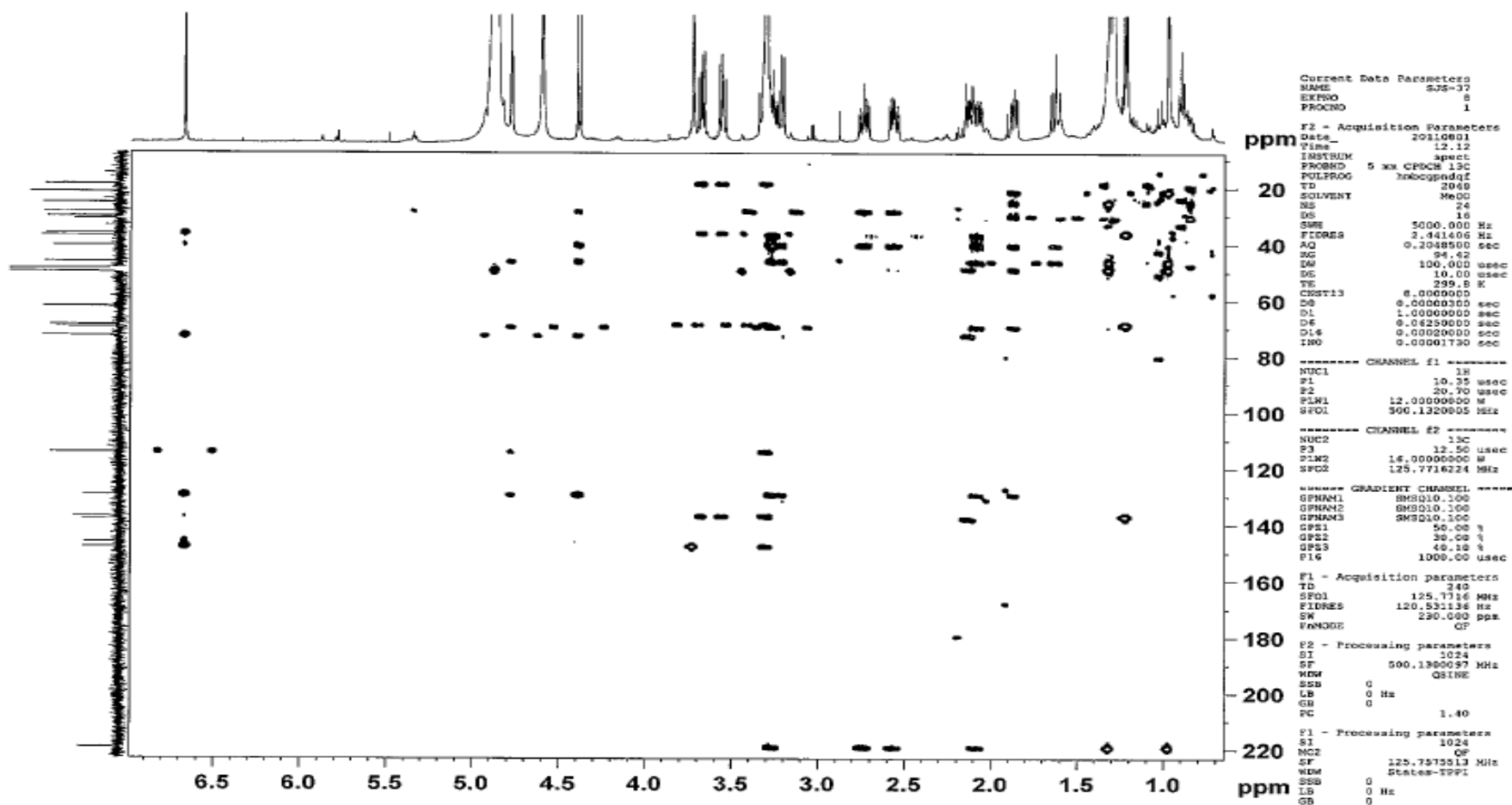
Figure S31 NOSEY of Lanceolatin D (4)
