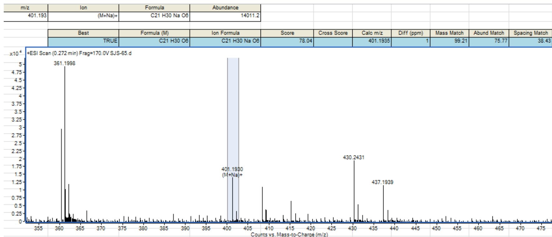
Figure S32 HR-ESI-MS of Lanceolatin E
