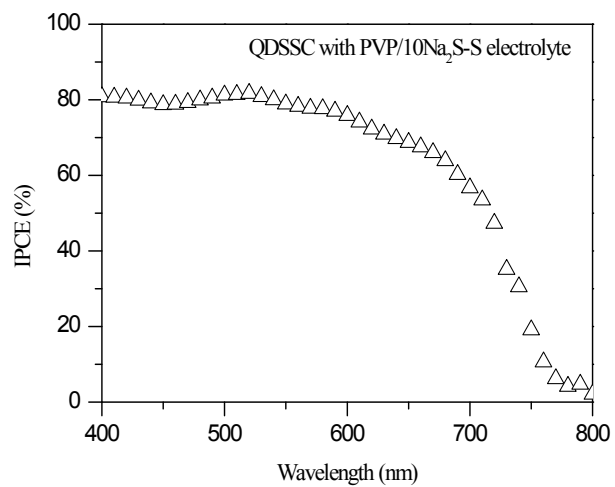
Fig. S1 IPCE spectral action response of the QDSSC from PVP/10Na 2 S-S electrolyte.
