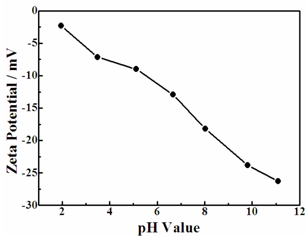
Fig. S2. Zeta potential plot of S3 sample at different pH value.
