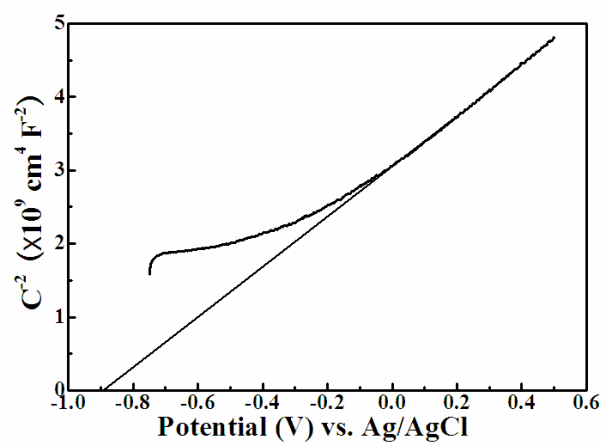
Fig. S3. Mott-Schottky plot for BiOCOOH electrode in the 0.1 mol L -1 Na 2 SO 4 solution.
