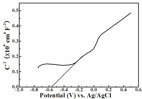
Fig. S4. Mott-Schottky plot for S3 electrode in the 0.1 mol L -1 Na 2 SO 4 solution.
