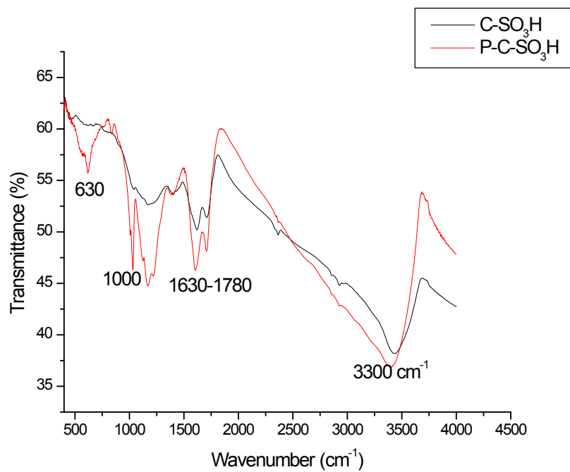
Fig. S2: FT-IR spectra of P-C-SO 3 H and C-SO 3 H
