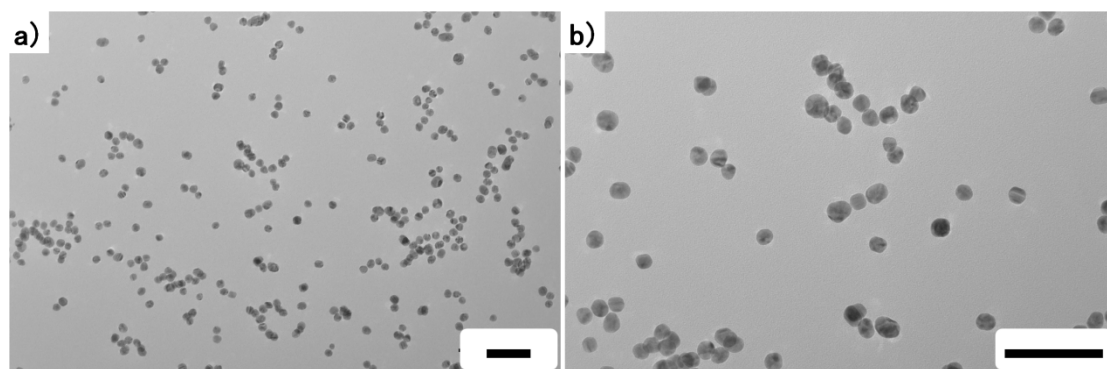
Fig.S1 TEM images of AuNPs. Scale bar: 100 nm.
