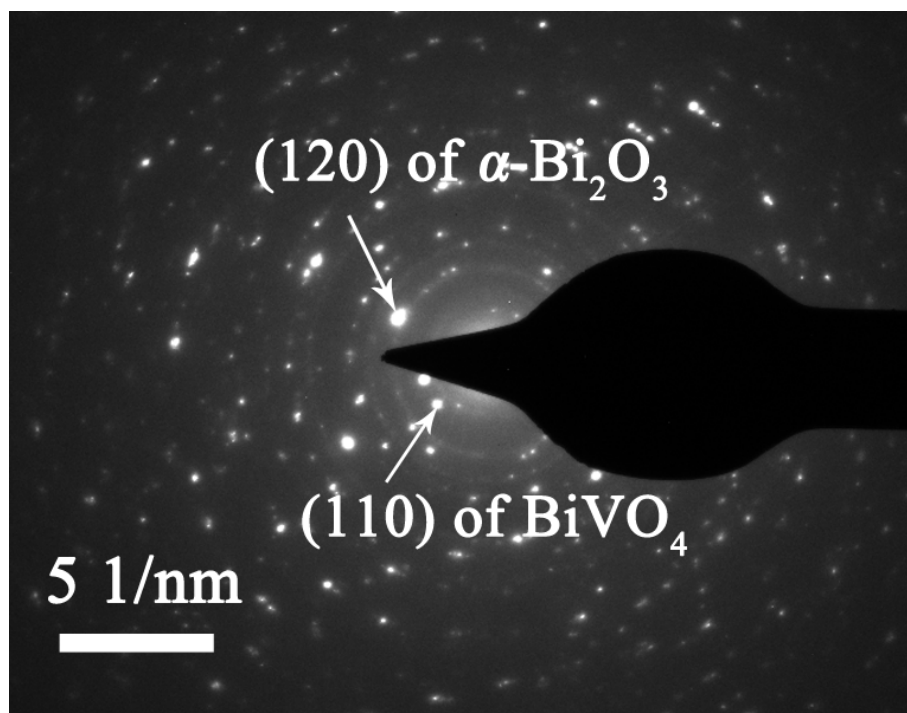
Fig. S1 SAED pattern taken at the surface of BQDs-BVNFs
