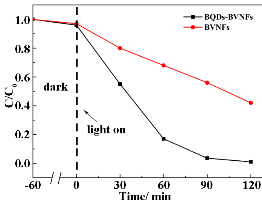
Fig. S2 Photocatalytic degradation of RhB under visible light without \text{H}_2\text{O}_2 .
