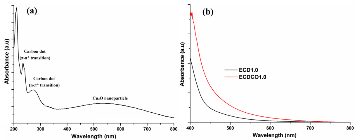
Fig. S1 Optical absorption spectra of (a) carbon dot reduced \text{Cu}_2\text{O} nanohybrid and (b) ECD1.0 and ECDCO1.0.
