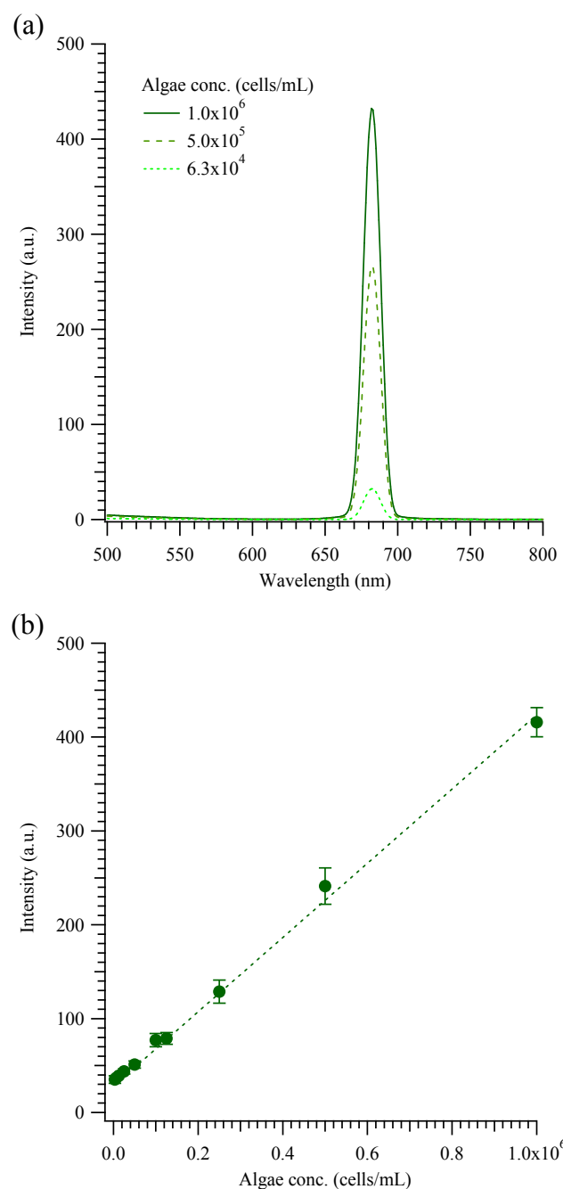
Figure S-1. (a) The emission spectrum and (b) the calibration curve of fluorescence intensity for the algae concentrations.
