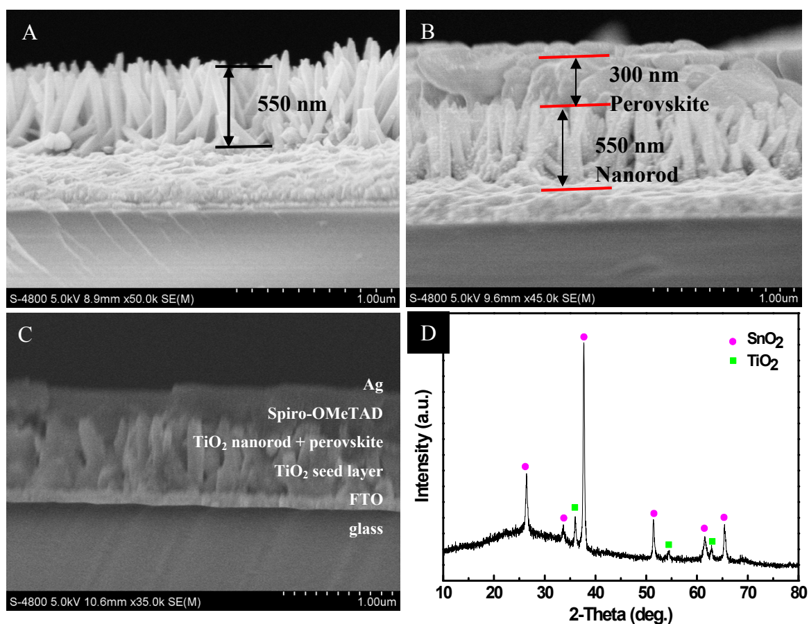
Fig. S1 (A) FESEM images of obtained \text{TiO}_2 nanorod grown on FTO substrate, (B) \text{CH}_3\text{NH}_3\text{PbI}_3 -deposited \text{TiO}_2 films, (C) full cell, and (D) XRD of \text{TiO}_2 nanorod grown on FTO substrate.
