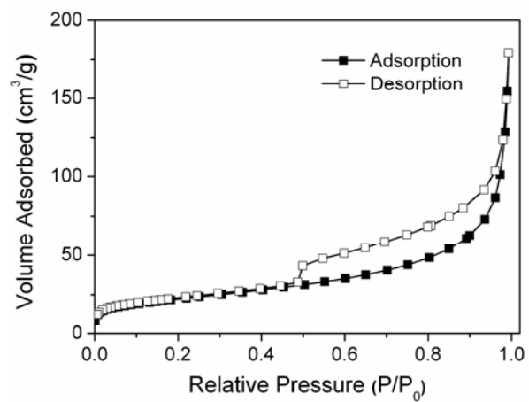
Fig. S1 N 2 adsorption–desorption isotherms of SnO 2 hollow nanospindles.
