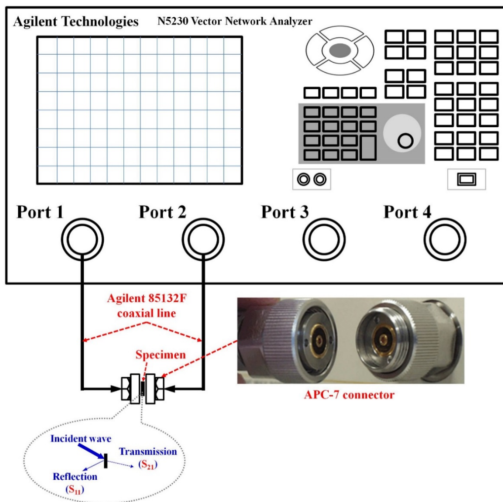
Fig. S11 Schematic of EMI shielding measurement setup.
