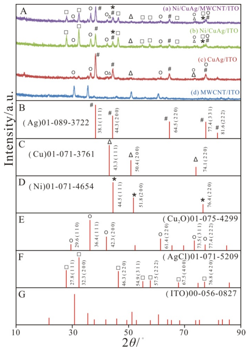
Fig. S1 (A) XRD spectra of different modified ITO electrodes. Standard XRD patterns: (B) Ag, (C) Cu, (D) Ni, (E) Cu 2 O, (F) AgCl, and (G) ITO, respectively.
