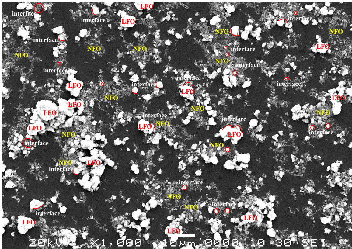
FIG.S2. SEM micrograph of 60%LFO-40%NFO composite
