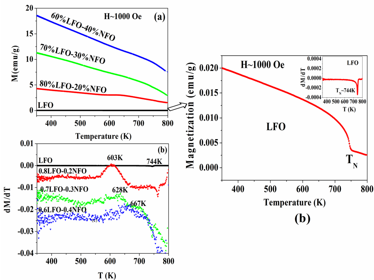
FIG.S1. (a) Temperature dependence magnetization of LFO and LFO-NFO composites at H \sim 1 kOe (b) Enlarge plot of temperature dependence magnetization of LFO at 1kOe plot with inset showing its derivative plot (c) dM/dT versus temperature plot
