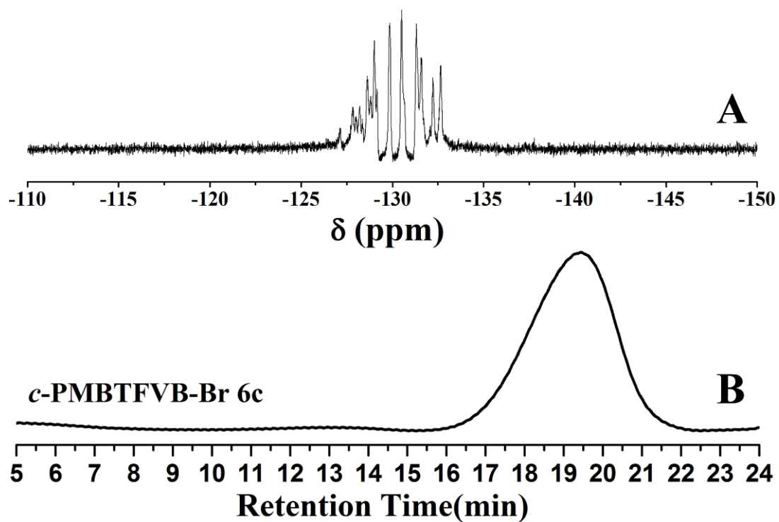
Figure S3. ^{19}\text{F} NMR spectrum (A) and GPC curve (B) of c -PMBTFVB-Br 6c .
