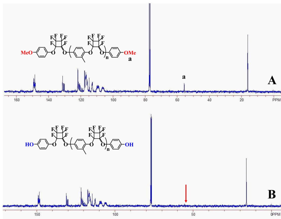
Figure S1. ^{13}\text{C} NMR spectra of MeO-PMBTFVB-OMe 2 (A) and HO-PMBTFVB-OH 3 (B) in \text{CDCl}_3 .
