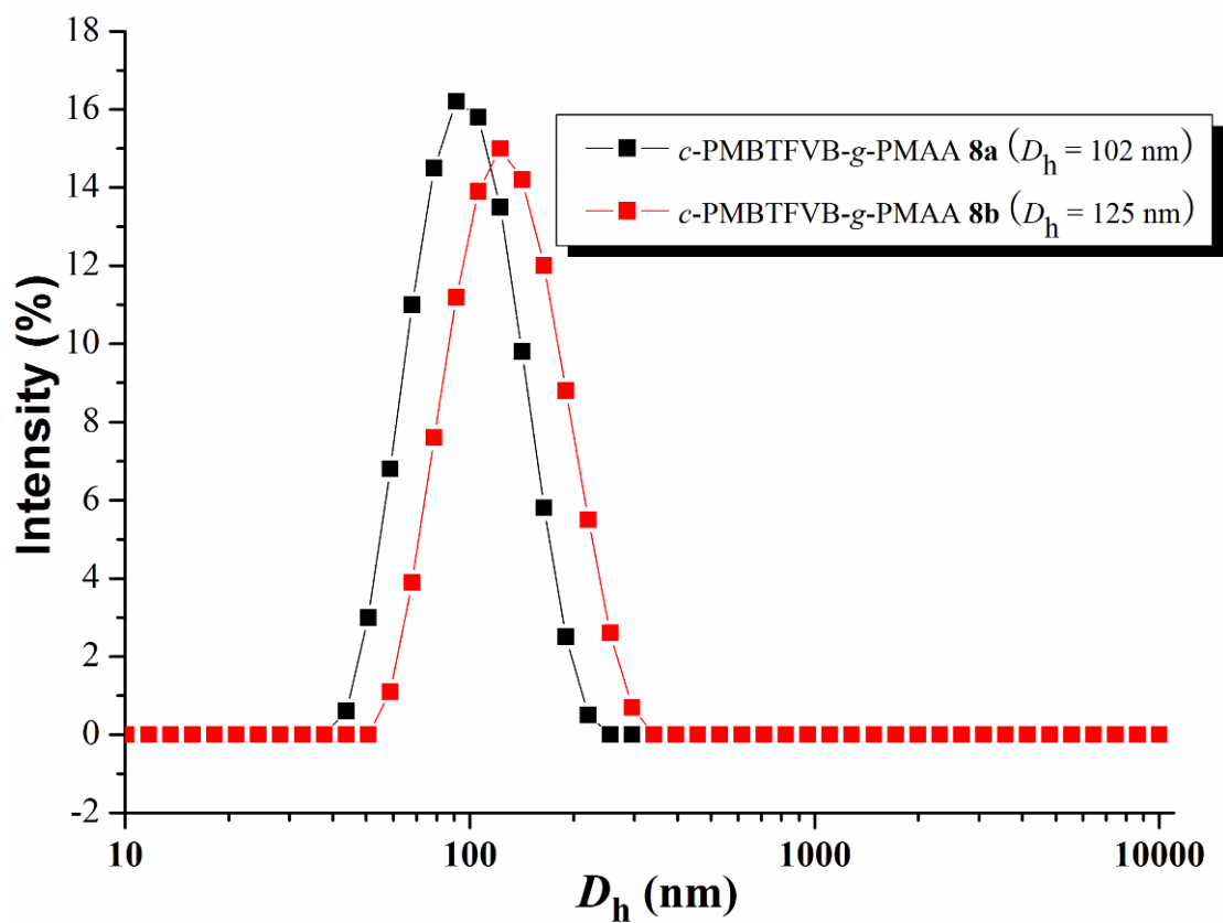
Figure S4. Hydrodynamic diameter distributions of micelles formed by c -PMBTFVB- g -PMAA 8a and 8b .
