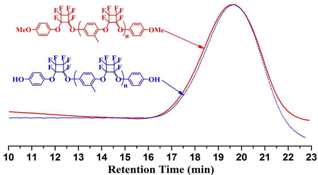
Figure S2. GPC traces of MeO-PMBTFVB-OMe 2 (red) and HO-PMBTFVB-OH 3 (blue) in THF.
