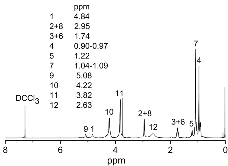
Fig. S2 1 H-NMR spectrum of BHIDU
