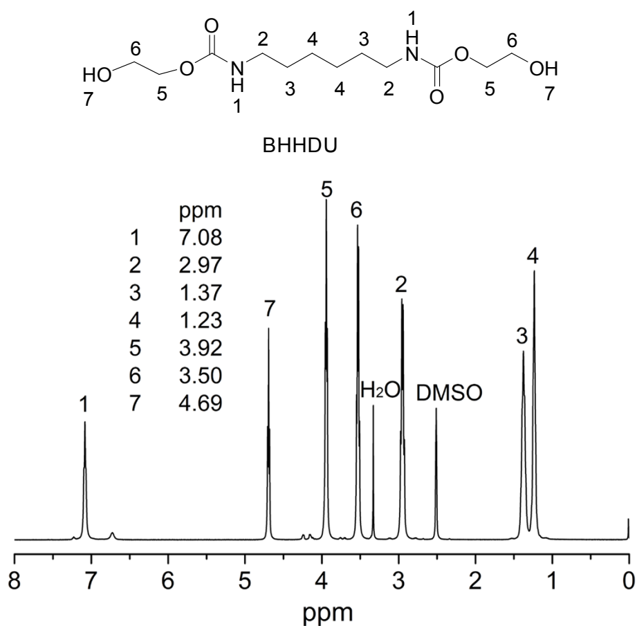
Fig. S1 ^1\text{H-NMR} spectrum of BHHDU
