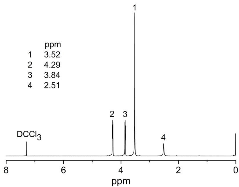
Fig. S3 1 H-NMR spectrum of BHPDU
