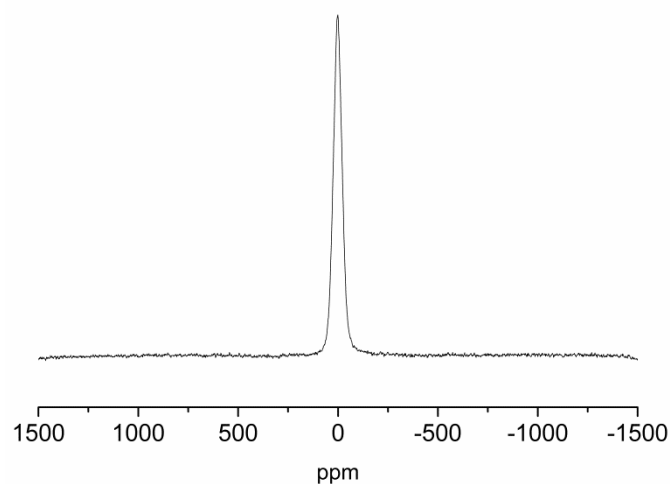
Figure S2. CP MAS 7 Li NMR spectra of initiator, Ph 2 Si(OLi) 2 .
