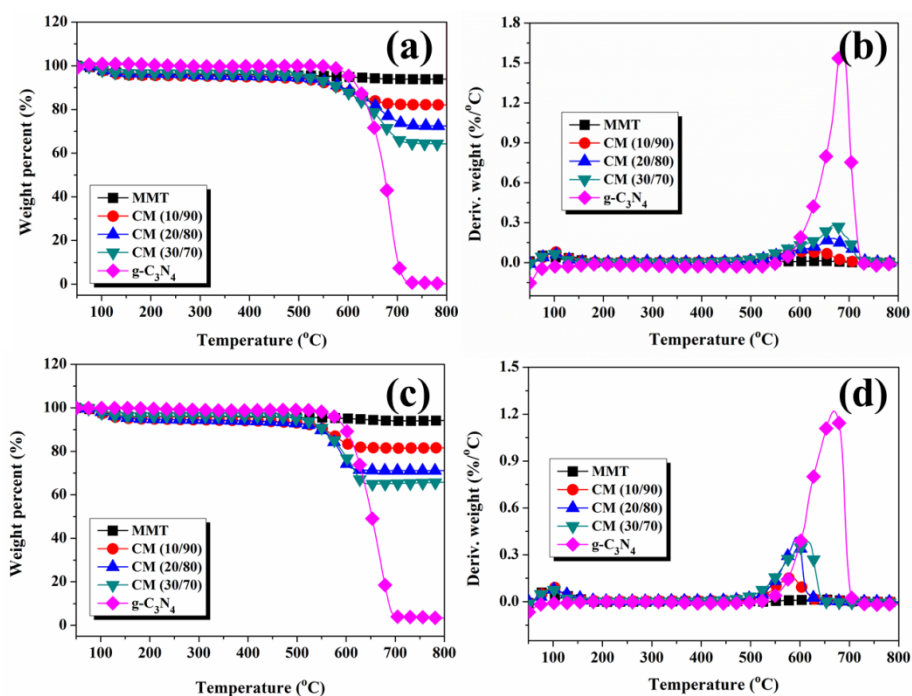
Figure 1S. TGA and DTG curves of g-C 3 N 4 , Na-MMT and their nanohybrids with different weight ratio under nitrogen (a, b) and air (c, d) conditions.
