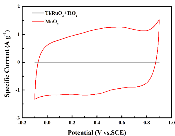
Fig. S1 Cyclic voltammetric curves of \text{Ti}/\text{RuO}_2+\text{TiO}_2 and \text{MnO}_2 at a scan rate of 5 \text{mV s}^{-1} .
